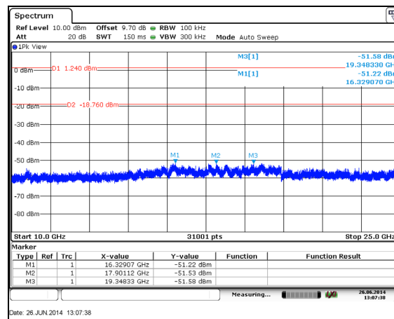
Figure 7.5.1.2-9: 10 GHz – 25 GHz – 2480 MHz
