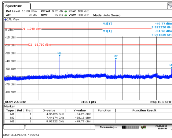
Figure 7.5.1.2-8: 2.5 GHz – 10 GHz – 2480 MHz
