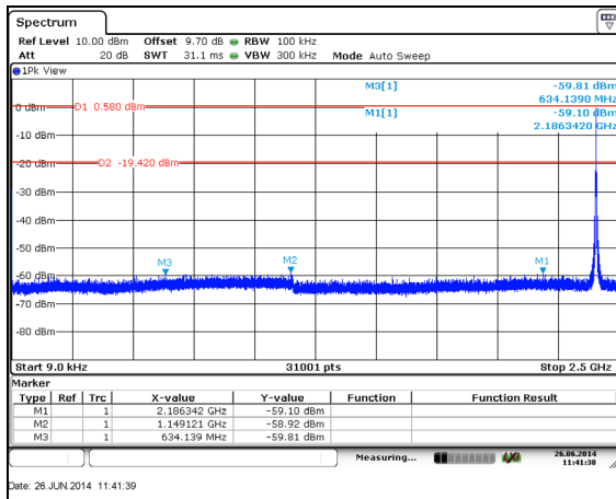
Figure 7.5.1.2-1: 9.0 kHz – 2.5 GHz – 2405 MHz
