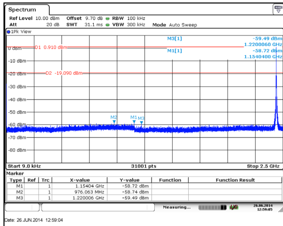
Figure 7.5.1.2-4: 9.0 kHz – 2.5 GHz – 2440 MHz
