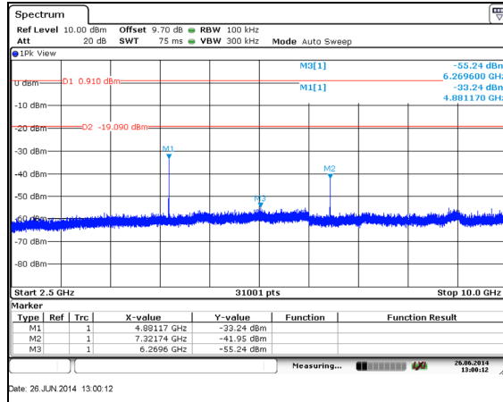
Figure 7.5.1.2-5: 2.5 GHz – 10 GHz – 2440 MHz
