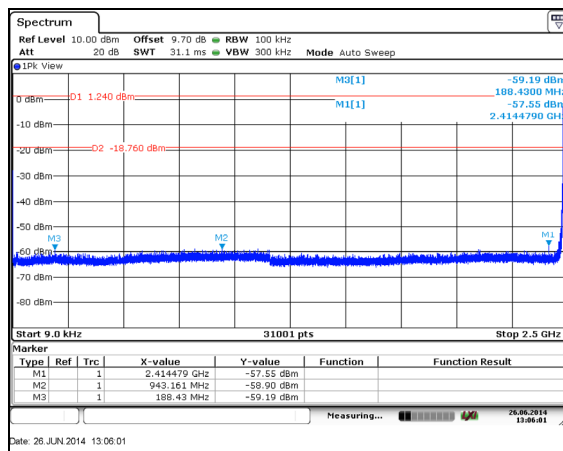
Figure 7.5.1.2-7: 9.0 kHz – 2.5 GHz – 2480 MHz
