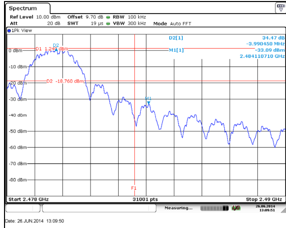
Figure 7.5.1.2-11: Upper Band-edge - 2480 MHz
