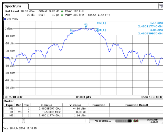
Figure 7.3.2-3: 6dB Bandwidth Plot – 2480 MHz
