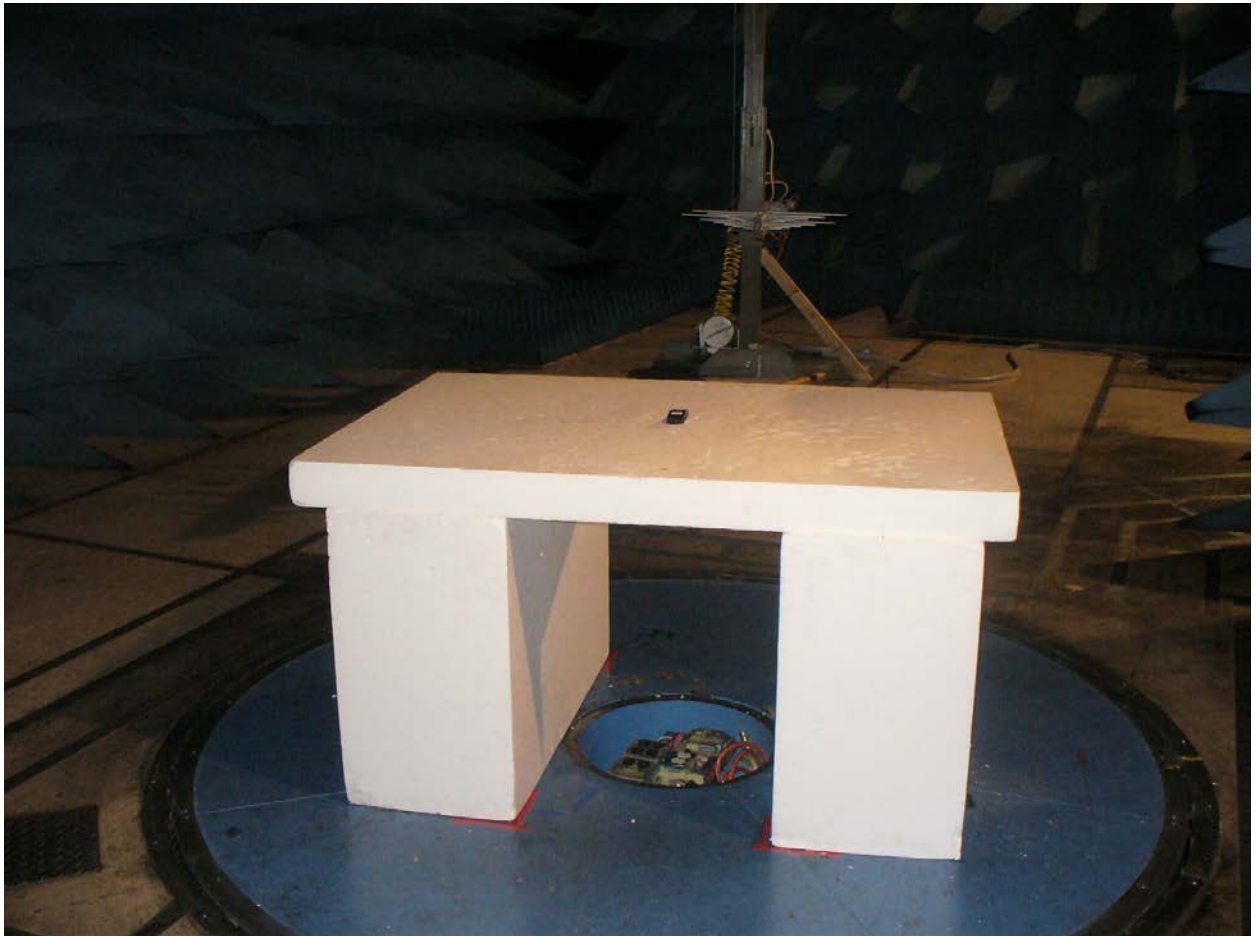
Figure 5: Radiated Emissions – Rear View (200 MHz – 1 GHz)
