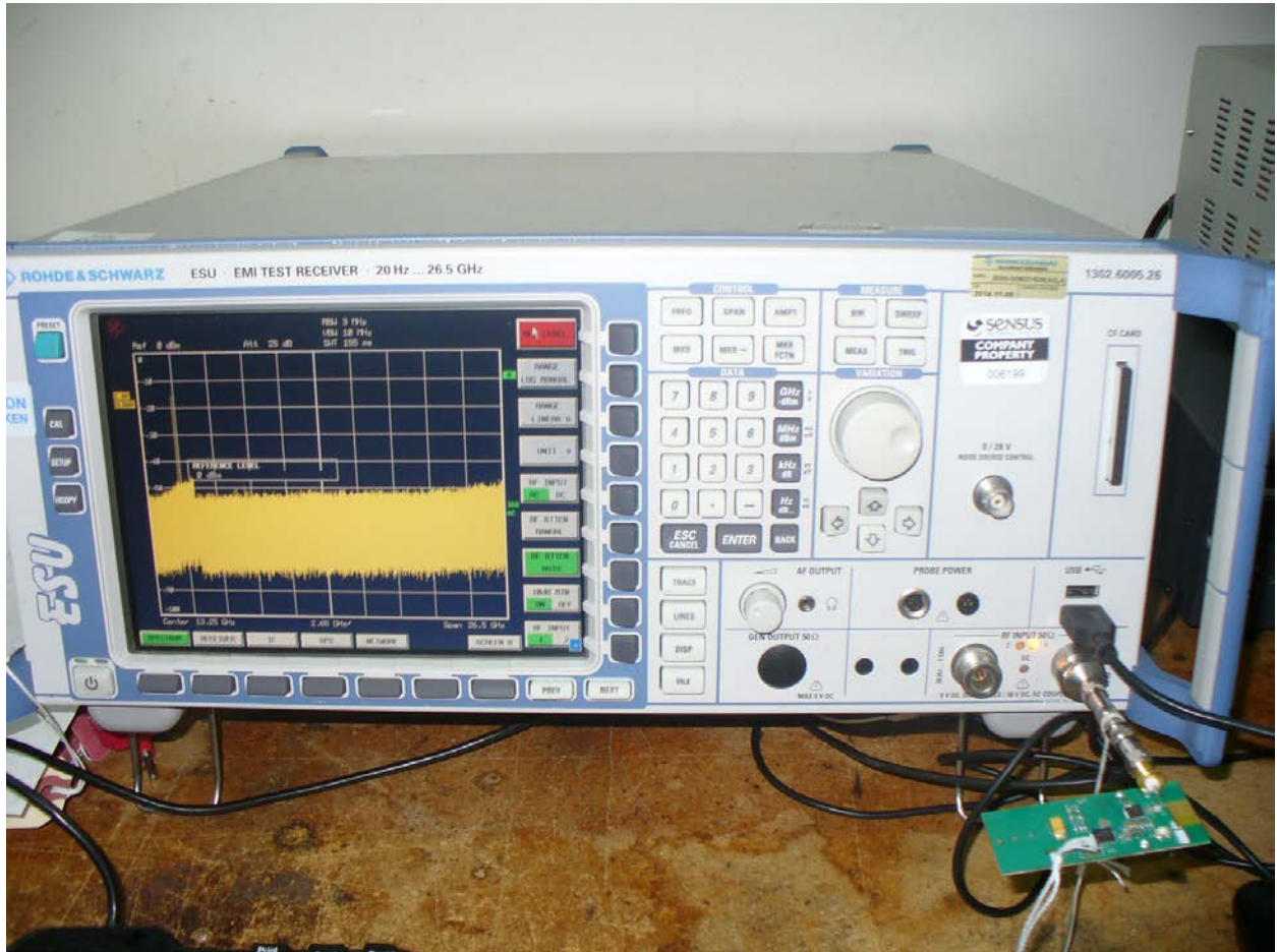
Figure 10: RF Conducted Measurements
