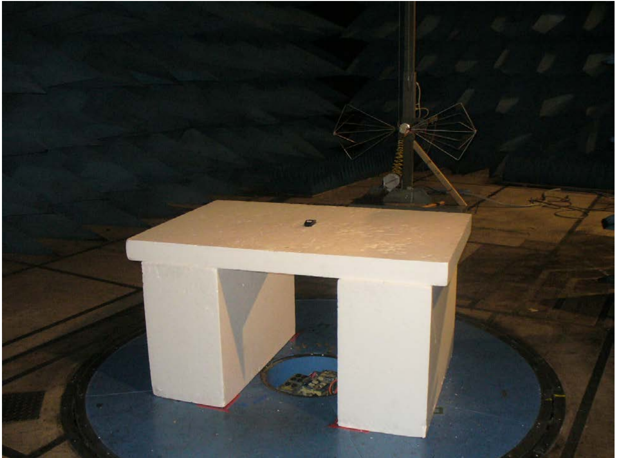
Figure 4: Radiated Emissions – Rear View (30MHz – 200 MHz)
