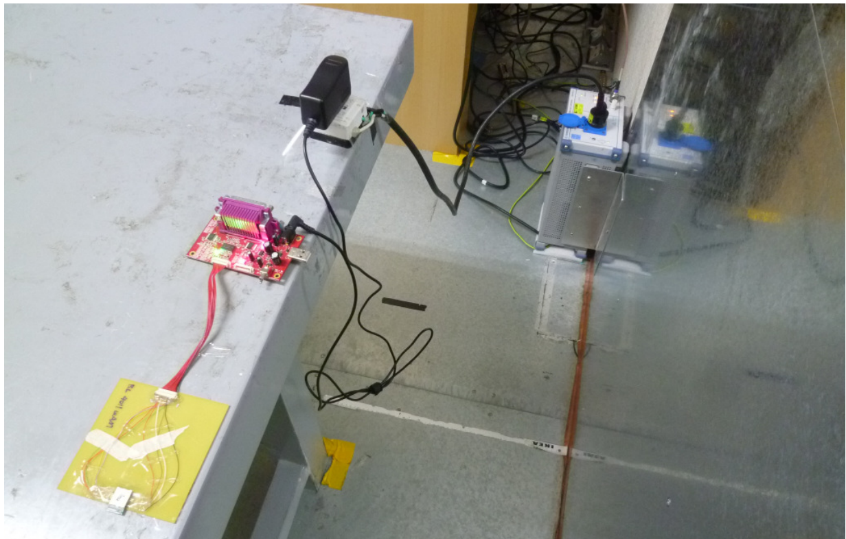
Photograph 9: Set-up for Mains Conducted testing Front
