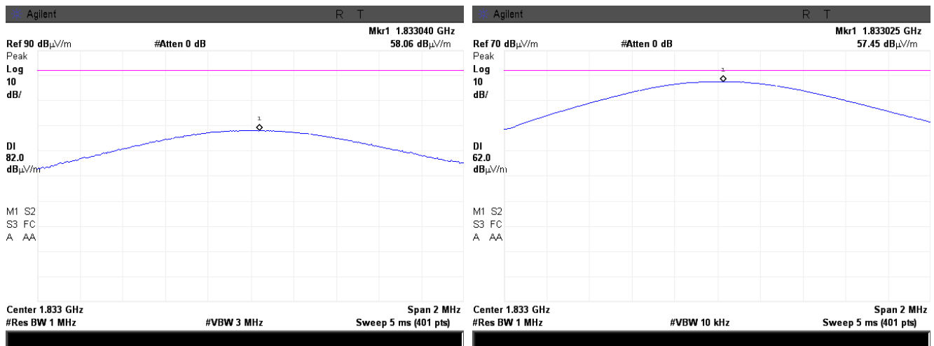
Plot 7.1.13 Radiated emission measurements at the second harmonic frequency
