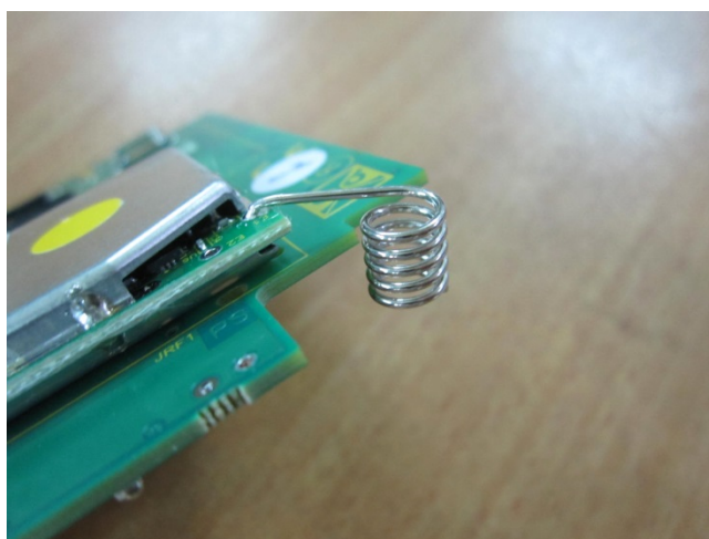
Photograph 7.5.1 Antenna assembly
