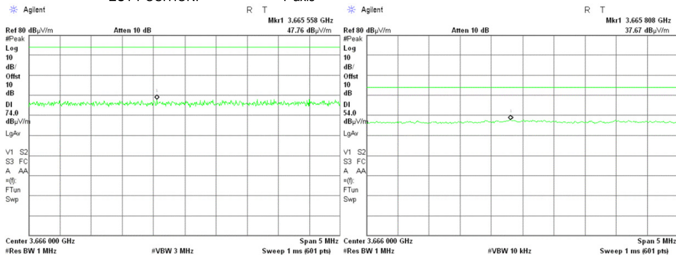
Plot 7.2.20 Radiated emission measurements at the fourth harmonic frequency
