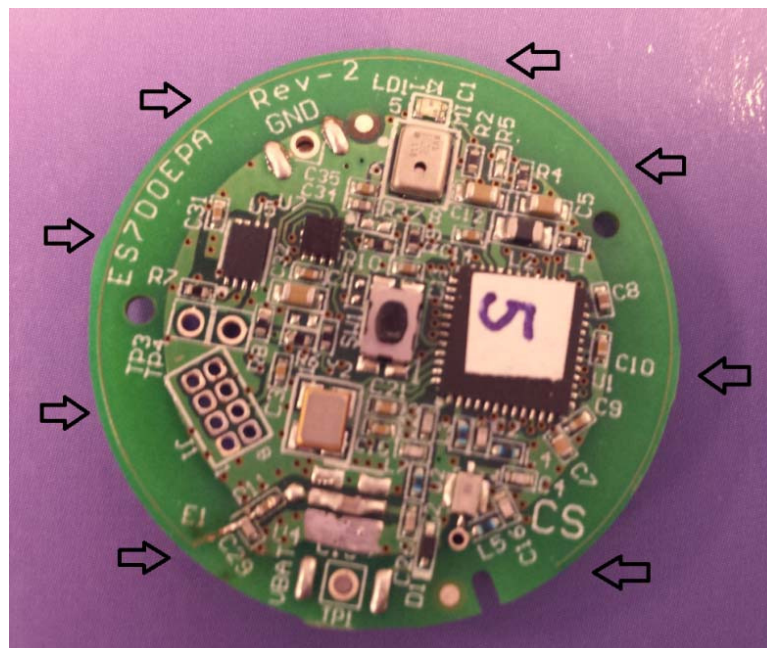
Photograph 7.4.1 Antenna assembly
