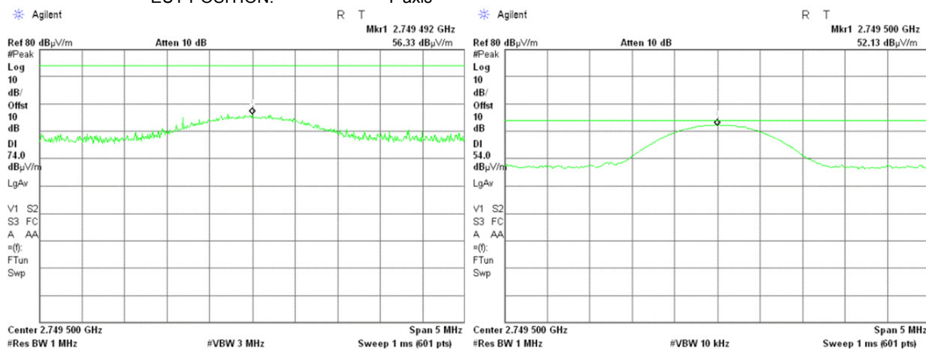
Plot 7.2.18 Radiated emission measurements at the third harmonic frequency
