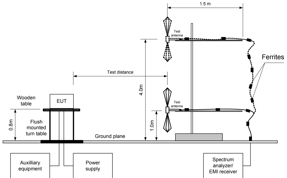
Figure 7.2.3 Setup for spurious emission field strength measurements above 1000 MHz
