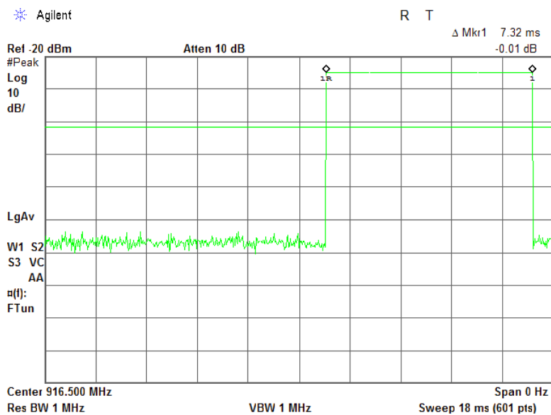
Plot 7.2.15 Transmission pulse duration
