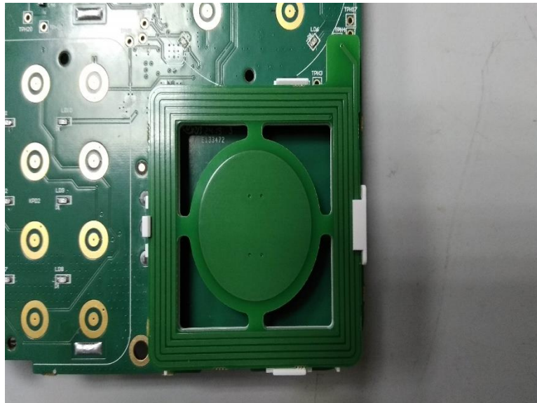
Photograph 7.5.1 Antenna assembly
