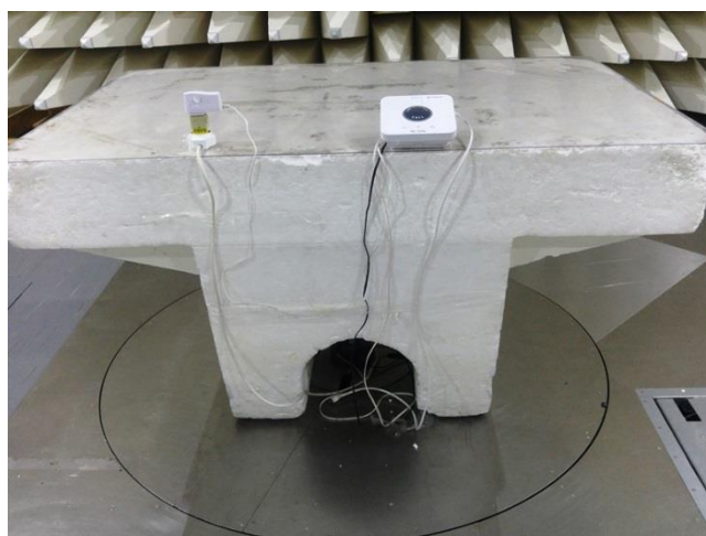
Photograph 8.2.2 Setup for radiated emission measurements, EUT cabling AC/DC adapter: UMEC
