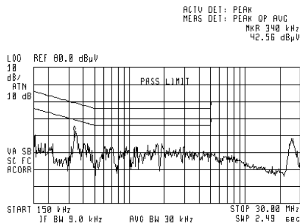
Plot 7.4.2 Conducted emission measurements
