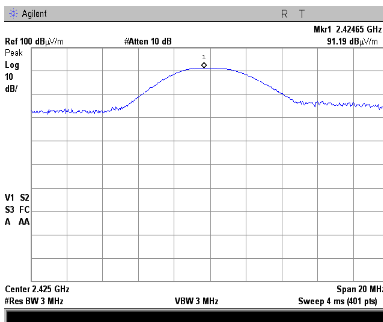
Plot 7.2.2 Field strength of carrier in vertical antenna polarization, EUT Y-axis position
