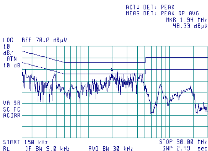
Plot 7.4.2 Conducted emission measurements
