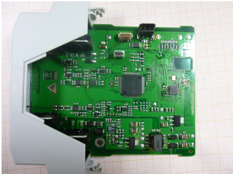
Photo 2: PCB front side view
