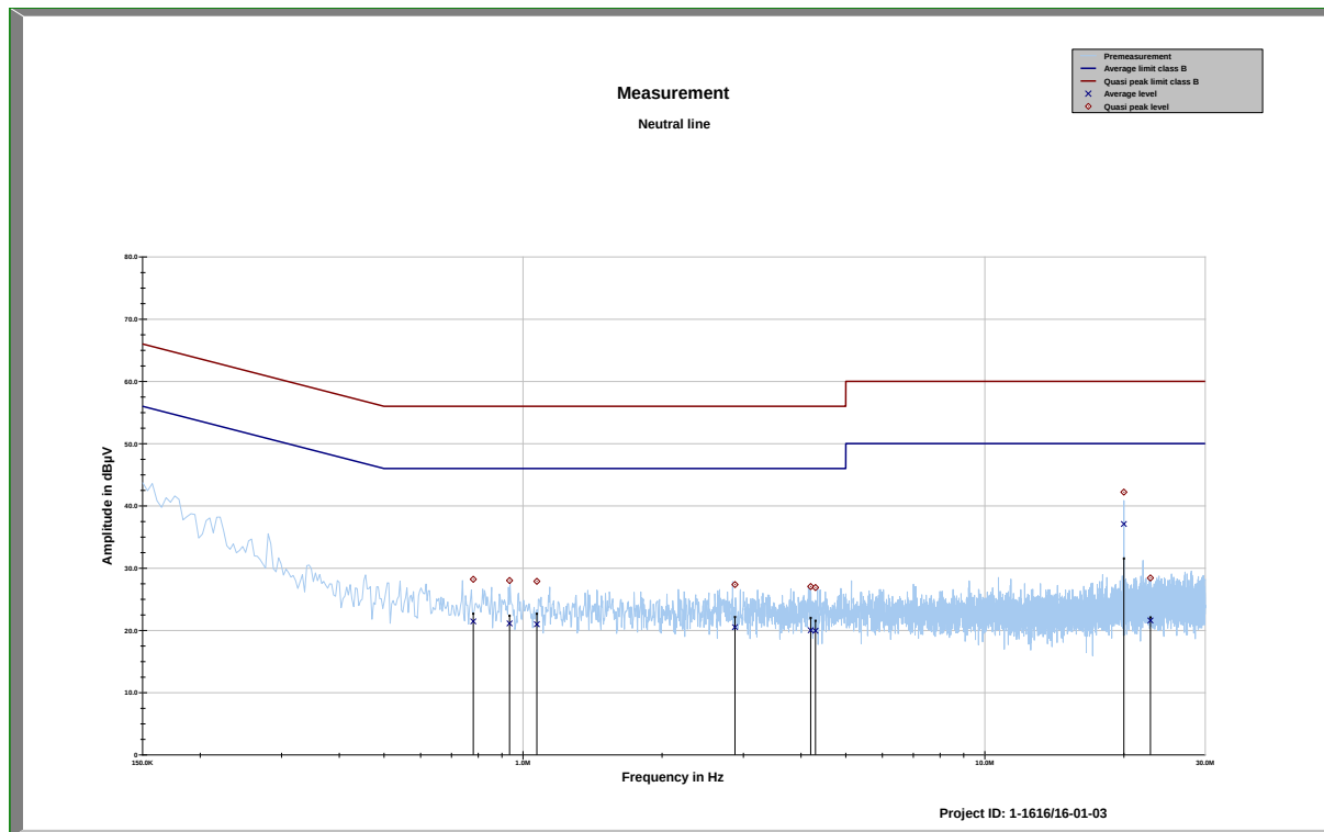
Plot 2: 150 kHz to 30 MHz, neutral line
