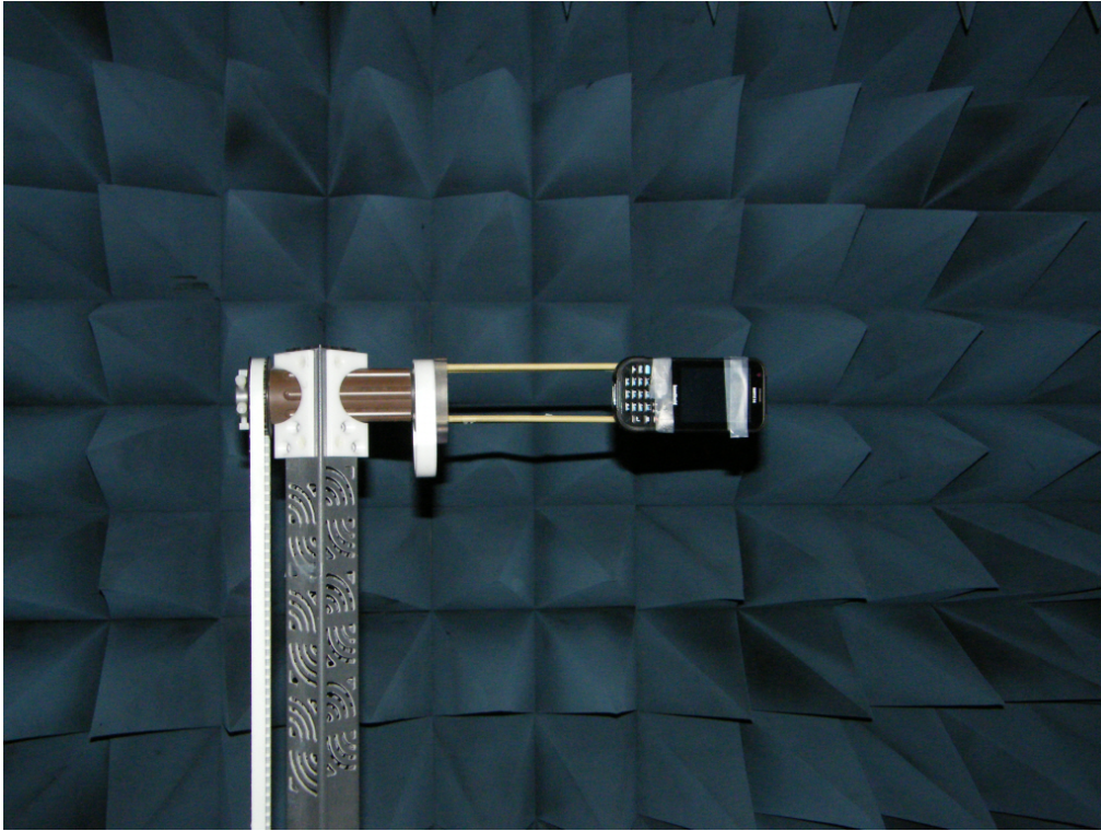
ERP & EIRP
