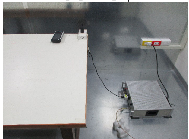
15_407_Conduction_Setup
