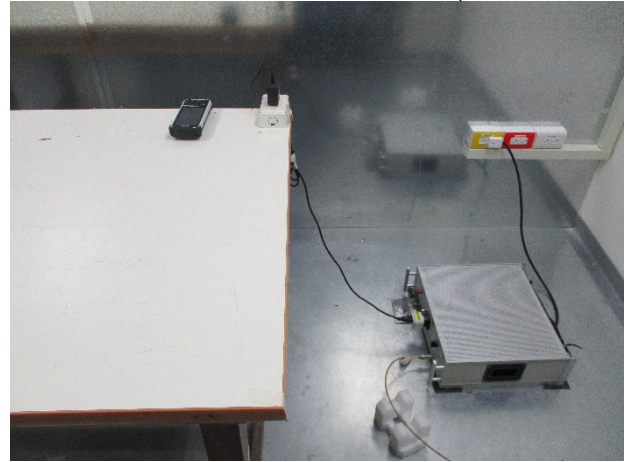
15_247_WLAN_Conduction_Setup
