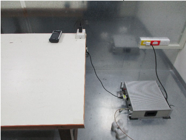
NFC_Conduction_Setup
