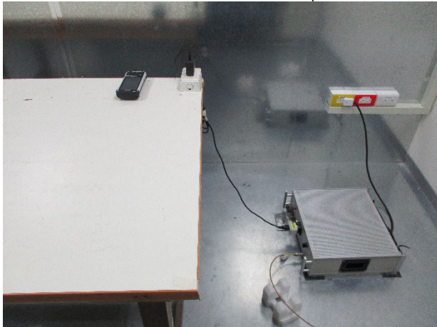
15_247_BT_Conduction_Setup
