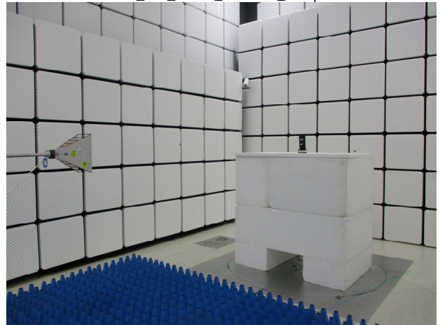
15_247_WLAN_Radiated_Setup
