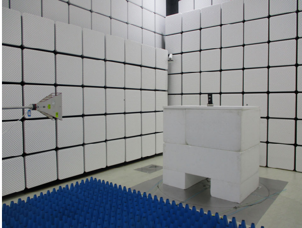
15_247_BLE_Radiated_Setup
