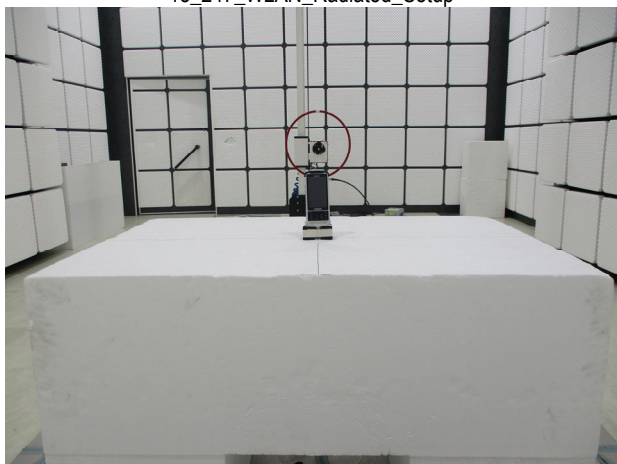
15_247_WLAN_Radiated_Setup
