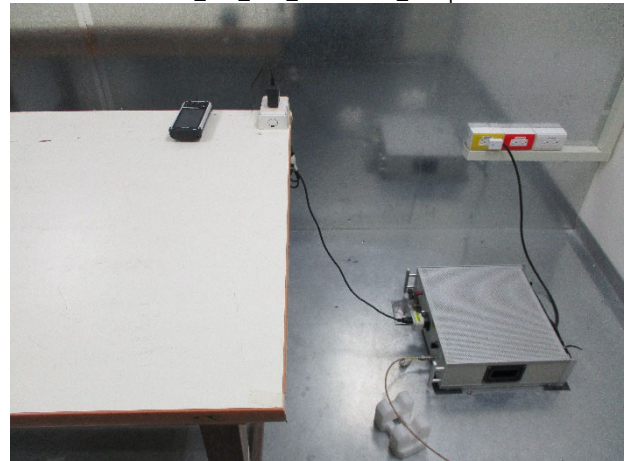
15_247_BLE_Conduction_Setup
