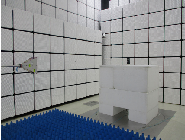
15_247_BT_Radiated_Setup
