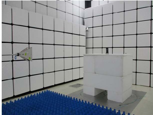
15_407_Radiated_Setup
