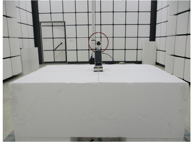
NFC_Radiated_Setup
