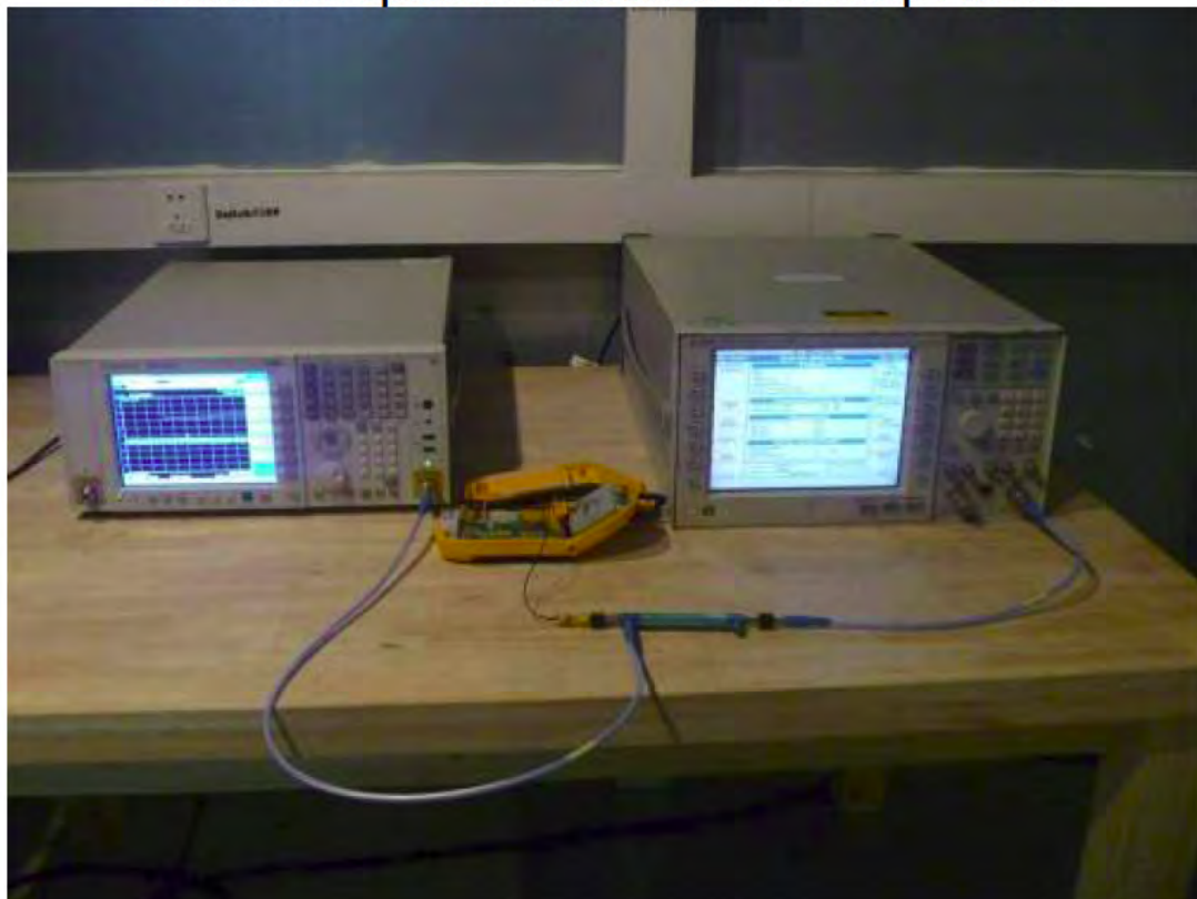
Conducted Spurious Emissions Test Setup Photos
