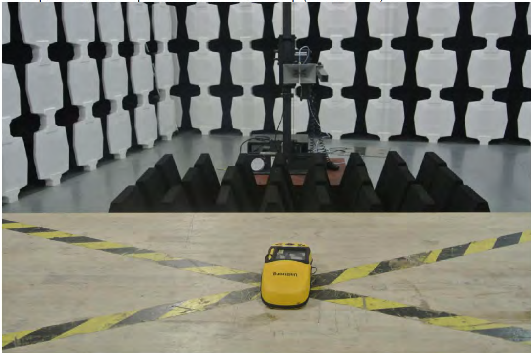
Description: Radiated Spurious Measurement Setup (Above 1GHz)
