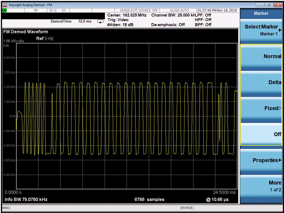
Figure 29- 162.025 MHz - 00001111
