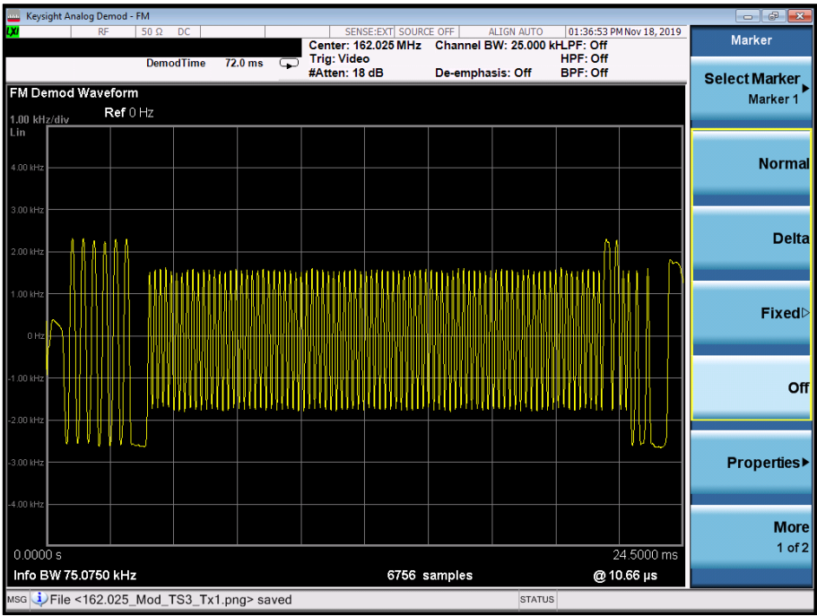
Figure 28 - 162.025 MHz - 01010101
