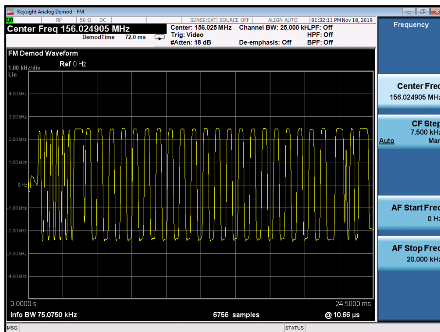
Figure 26- 156.025 MHz - 00001111
