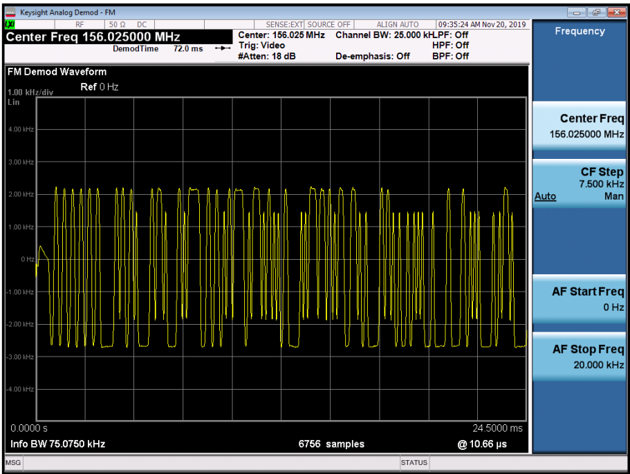
Figure 27- 156.025 MHz - PRBS
