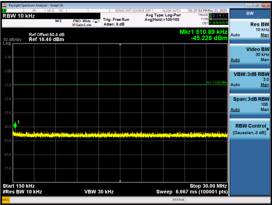
Figure 9 - Tx1, 156.025 MHz - 150 kHz to 30 MHz
