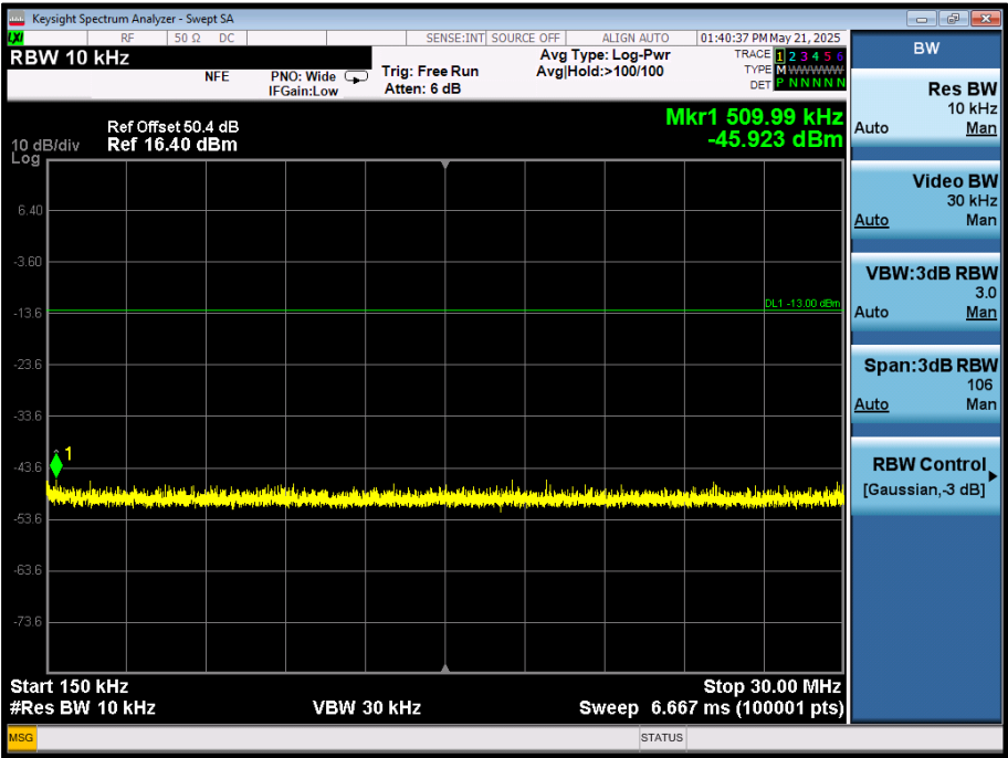
Figure 10 - Tx1, 162.025 MHz - 150 kHz to 30 MHz
