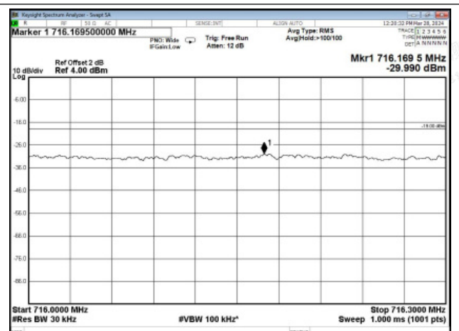
Lower 700MHz band CDMA UL Right Side 10dB Above AGC
