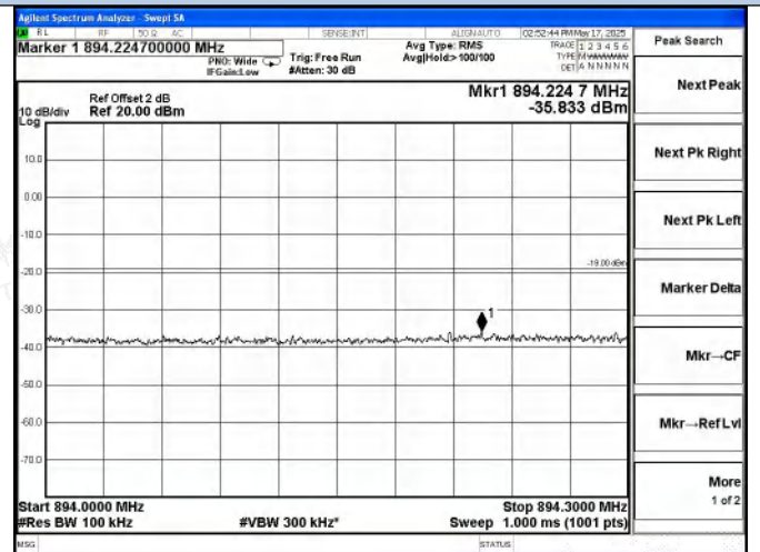
Cellular Band DL-CDMA Right Side AGC+5.5dB
