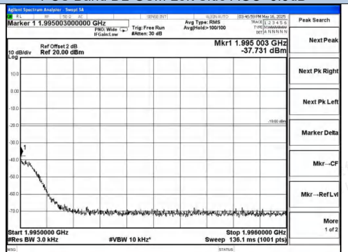
PCS Band DL-GSM Right Side AGC+5.5dB
