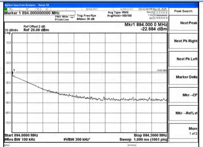
Cellular Band DL-GSM Right Side AGC+5.5dB
