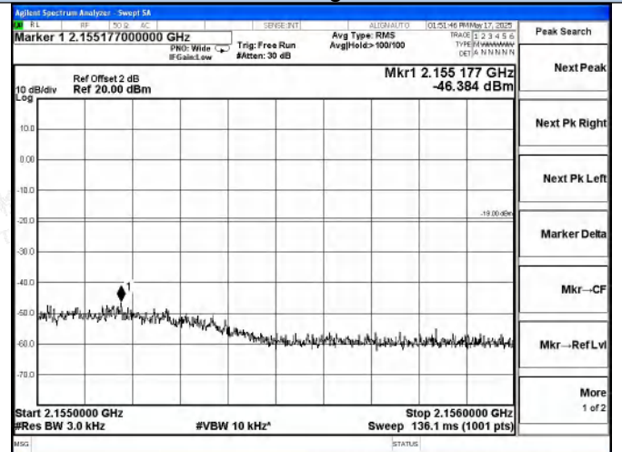
AWS Band DL-CDMA Left Side AGC+5.5dB
