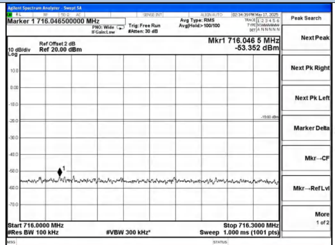
Lower 700 Band UL-CDMA Right Side AGC+5.5dB
