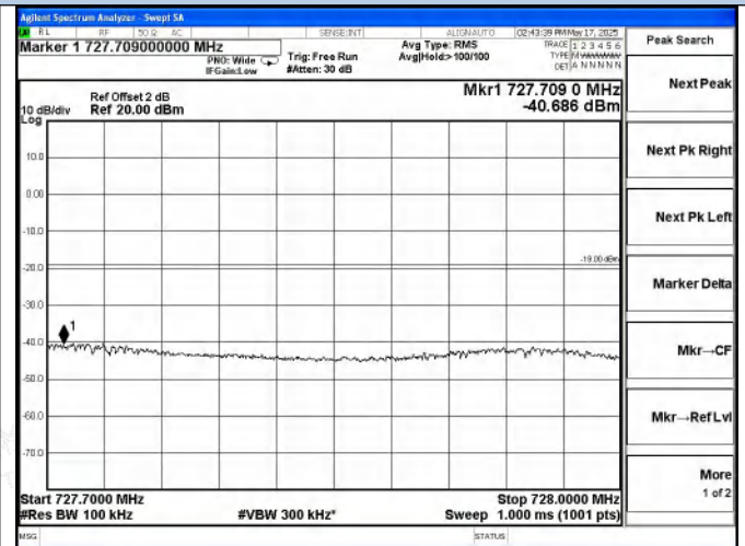
Lower 700 Band DL-CDMA Left Side AGC+5.5dB
