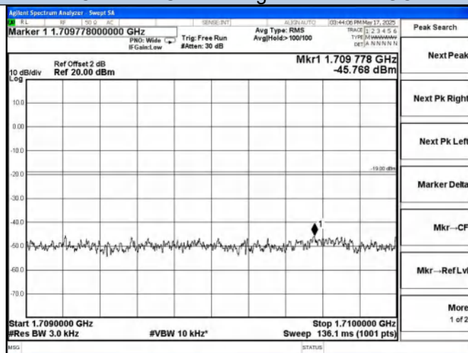
AWS Band UL-LTE Left Side Pre AGC
