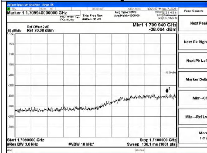
AWS Band UL-CDMA Left Side Pre AGC
