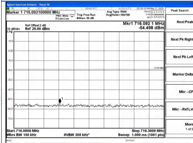
Lower 700 Band UL-CDMA Right Side Pre AGC
