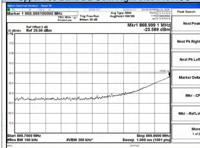
Cellular Band DL-GSM Left Side Pre AGC
