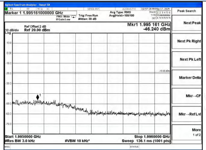
PCS Band DL-CDMA Right Side AGC+5.5dB
