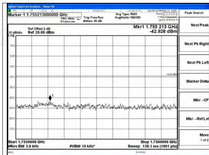
AWS Band UL-LTE Right Side Pre AGC
