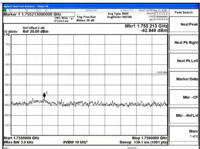
AWS Band UL-LTE Right Side AGC+5.5dB
