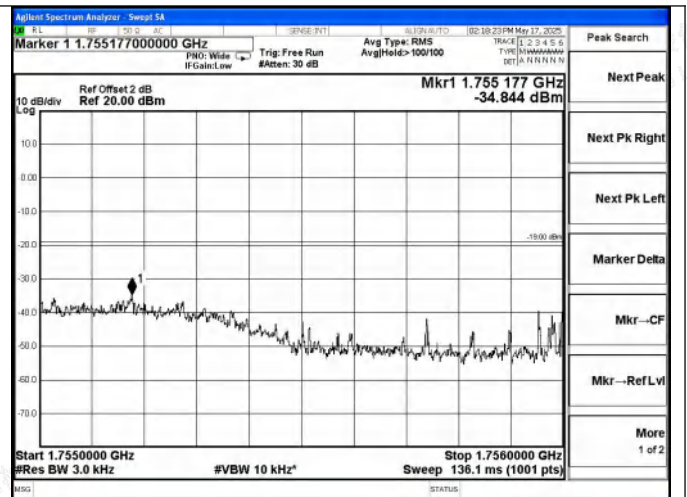
AWS Band UL-CDMA Right Side AGC+5.5dB
