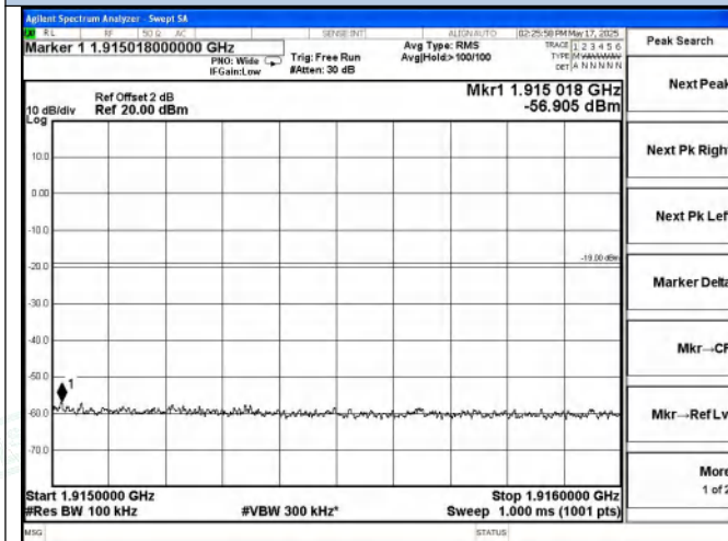
PCS Band UL-CDMA Right Side Pre AGC
