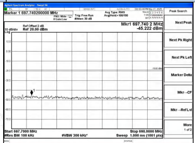
Lower 700 Band UL-CDMA Left Side AGC+5.5dB
