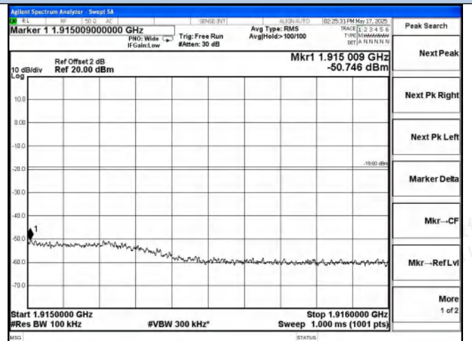
PCS Band UL-CDMA Right Side AGC+5.5dB
