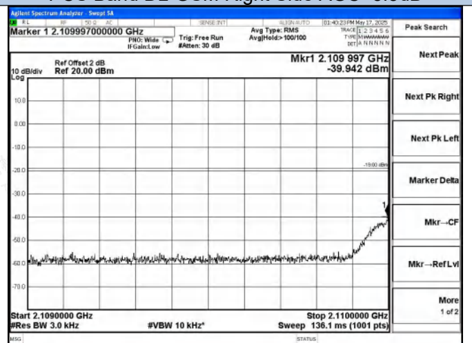
AWS Band DL-GSM Left Side AGC+5.5dB
