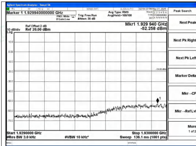
PCS Band DL-CDMA Left Side Pre AGC
