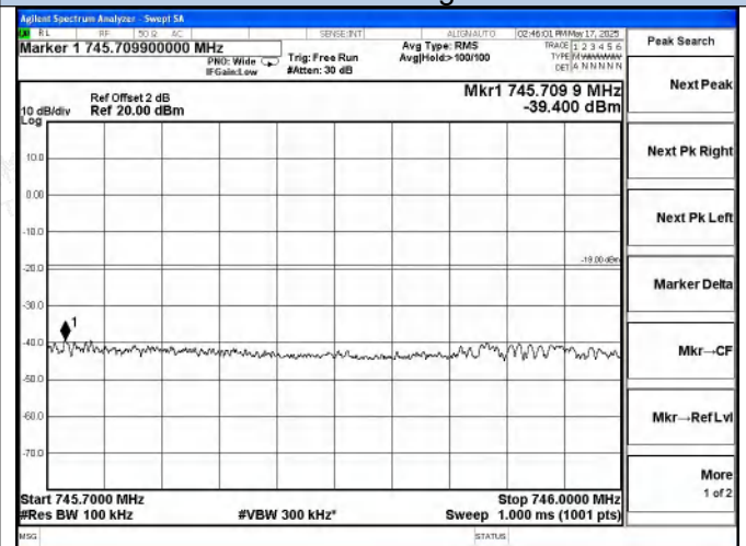
Upper 700 Band DL-CDMA Left Side AGC+5.5dB
