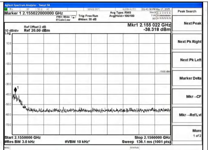
AWS Band DL-GSM Right Side AGC+5.5dB
