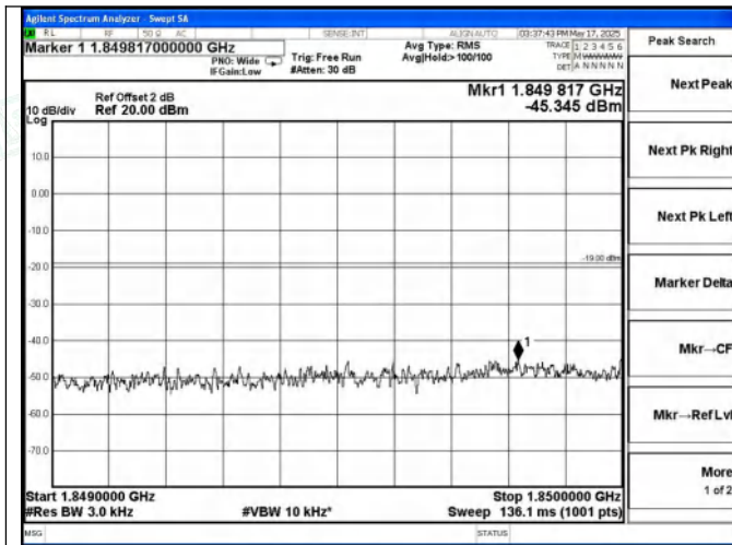
PCS Band UL-LTE Left Side Pre AGC
