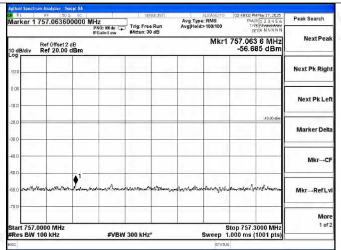
Upper 700 Band DL-CDMA Right Side AGC+5.5dB
