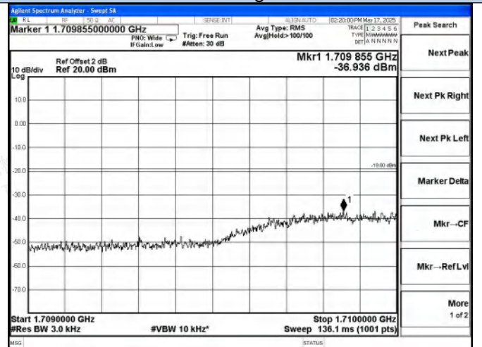
AWS Band UL-CDMA Left Side AGC+5.5dB
