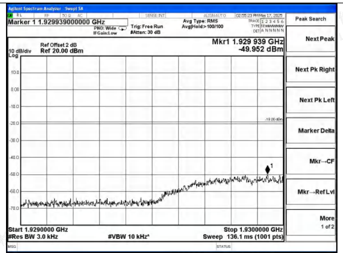
PCS Band DL-CDMA Left Side AGC+5.5dB
