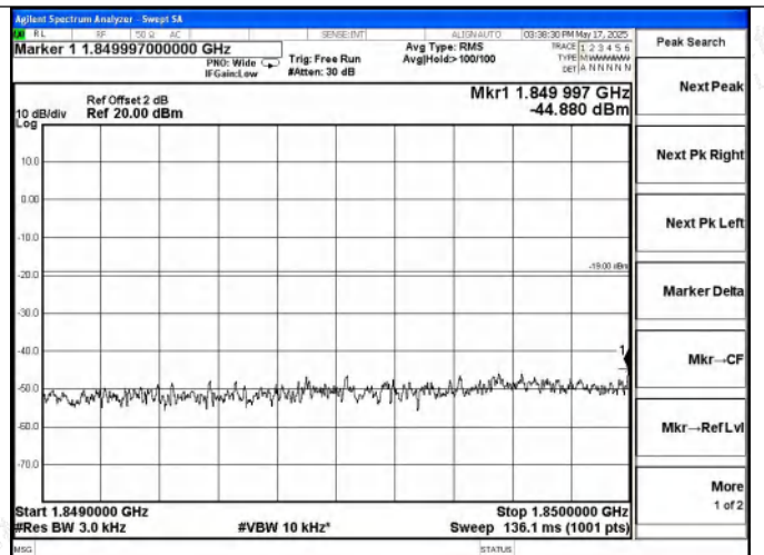
PCS Band UL-LTE Left Side AGC+5.5dB
