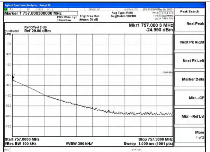
Upper 700 Band DL-GSM Right Side AGC+5.5dB
