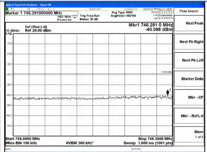
Lower 700 Band DL-CDMA Right Side AGC+5.5dB
