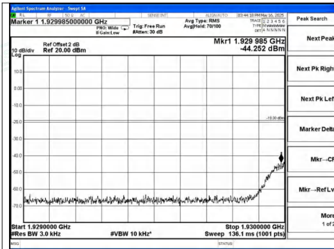
PCS Band DL-GSM Left Side Pre AGC
