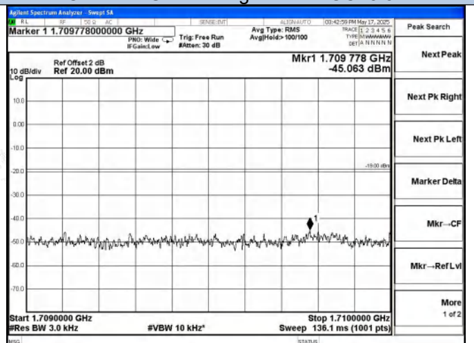
AWS Band UL-LTE Left Side AGC+5.5dB
