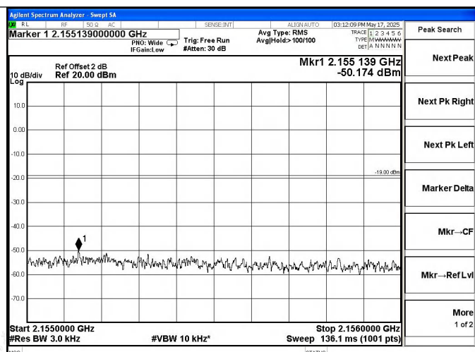
AWS Band DL-LTE Right Side AGC+5.5dB
