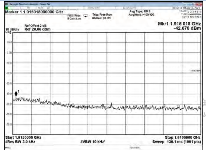
PCS Band UL-CDMA Right Side AGC+10dB
