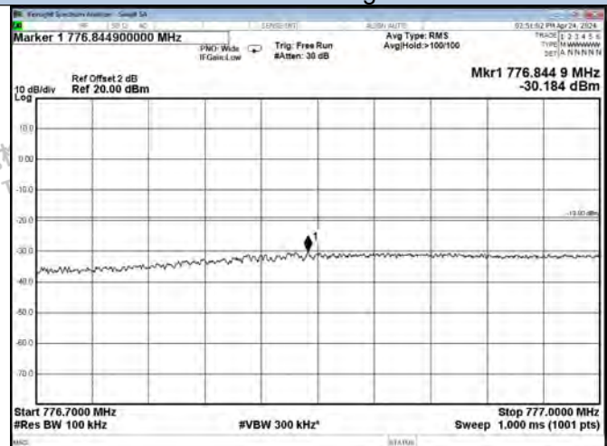
Upper 700 Band UL-CDMA Left Side AGC+10dB
