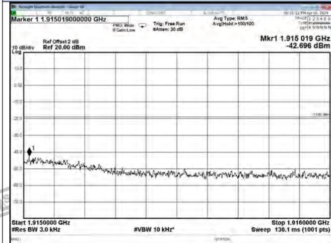
PCS Band UL-CDMA Right Side Pre AGC
