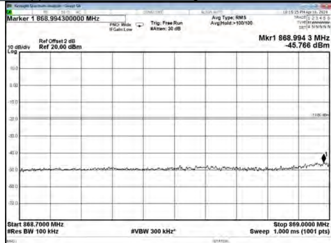
Cellular Band DL-LTE Left Side AGC+10dB
