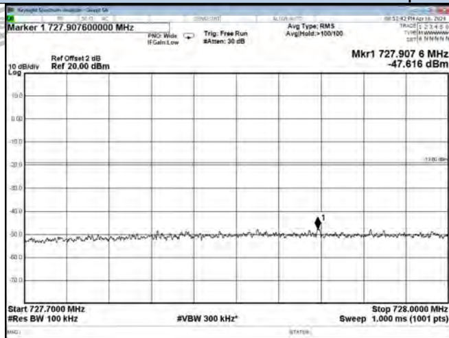
Lower 700 Band DL-CDMA Left Side Pre AGC
