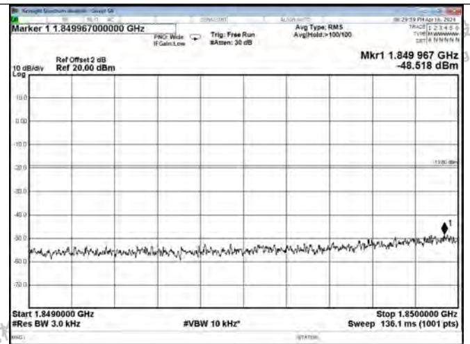
PCS Band UL-CDMA Left Side AGC+5.5dB
