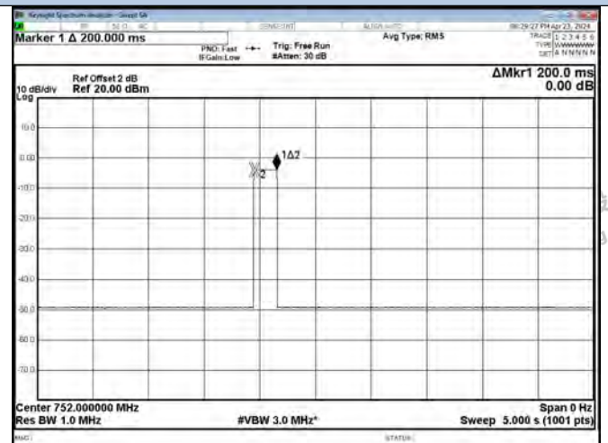
Detection Time-Upper 700 Band DL
