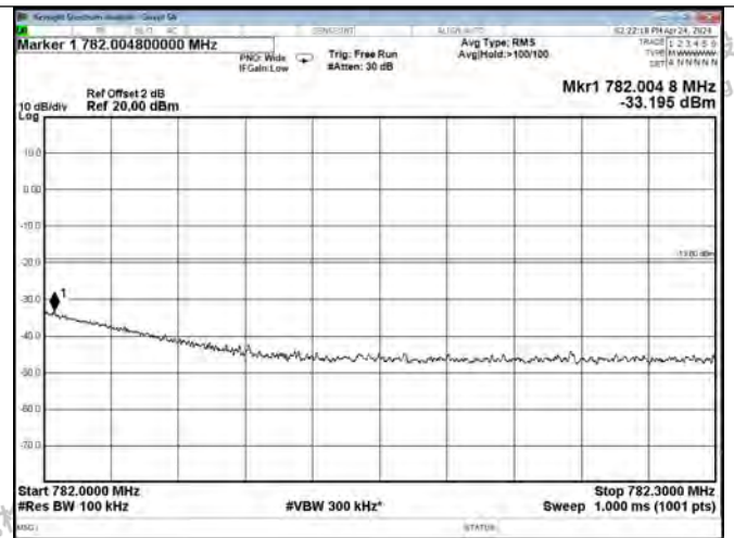
Upper 700 Band UL-GSM Right Side AGC+10dB
