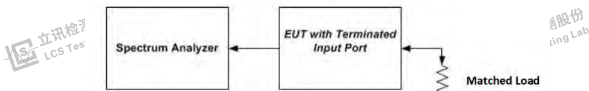
Figure 2 – Noise limit test setup
