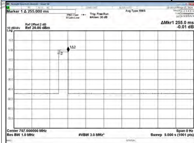
Detection Time-Lower 700 Band UL
