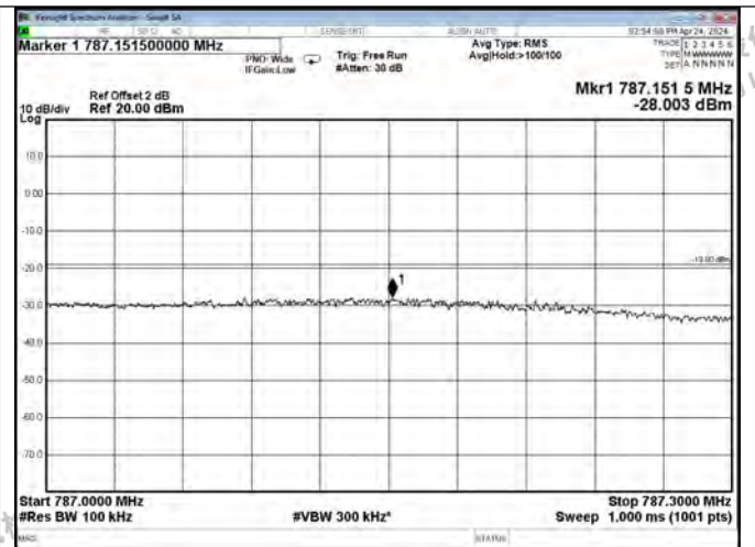
Upper 700 Band UL-CDMA Right Side AGC+10dB
