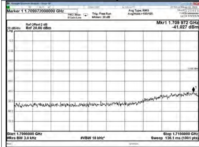
AWS Band UL-CDMA Left Side Pre AGC
