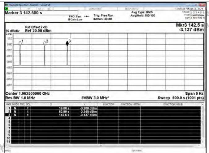
Restarting Time-PCS Band DL
