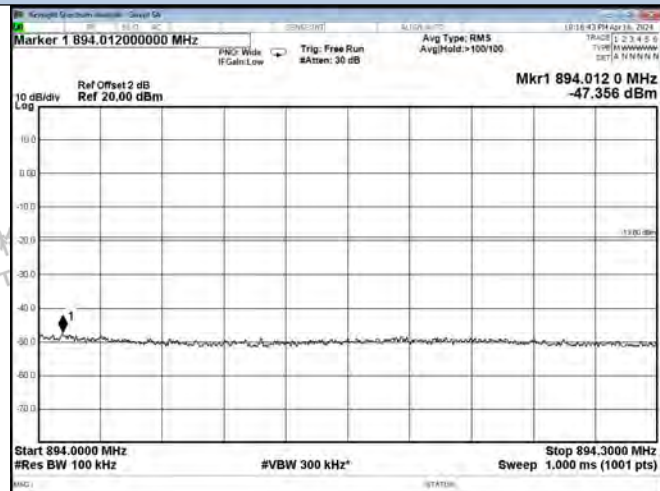
Cellular Band DL-LTE Right Side AGC+10dB
