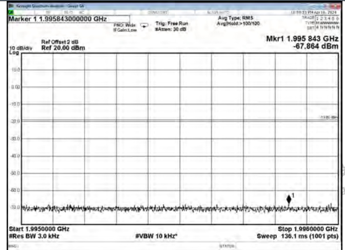
PCS Band DL-LTE Right Side AGC+10dB
