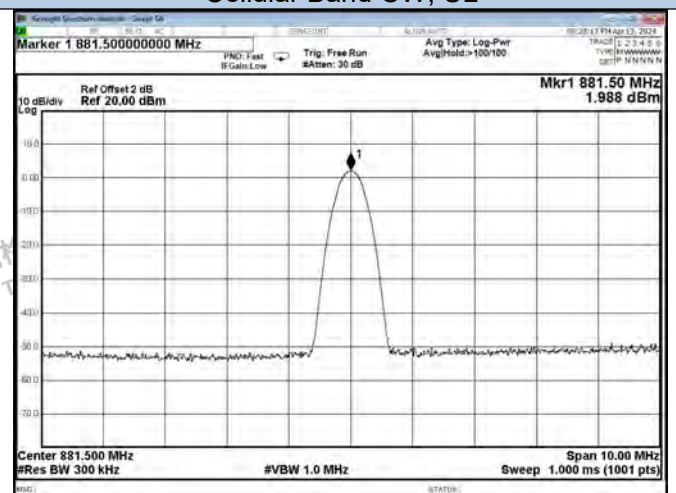
Cellular Band CW, DL
