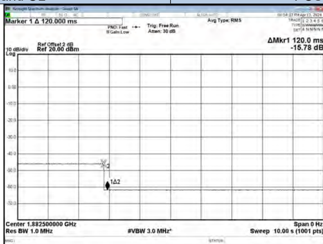
PCS Band Variable Uplink Noise Timing
