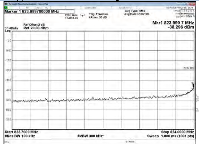
Cellular Band UL-GSM Left Side AGC+10dB
