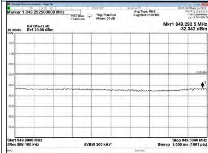
Cellular Band UL-CDMA Right Side Pre AGC
