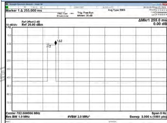
Detection Time-Upper 700 Band UL
