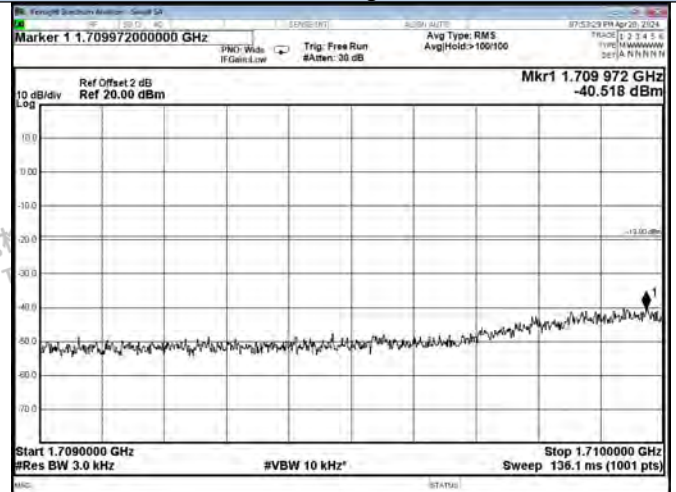
AWS Band UL-CDMA Left Side AGC+10dB
