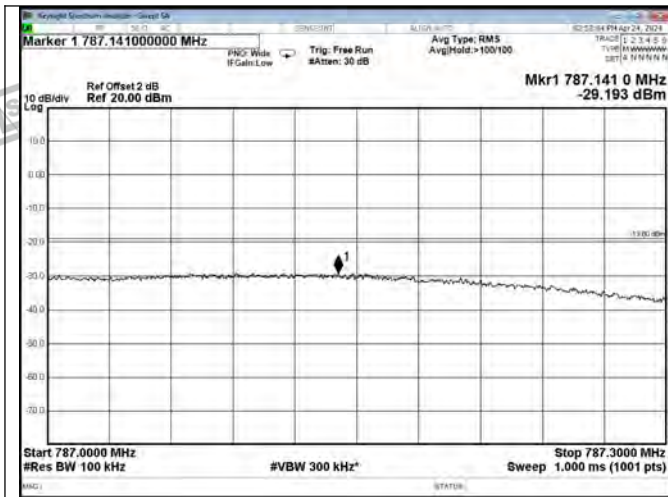
Upper 700 Band UL-CDMA Right Side Pre AGC
