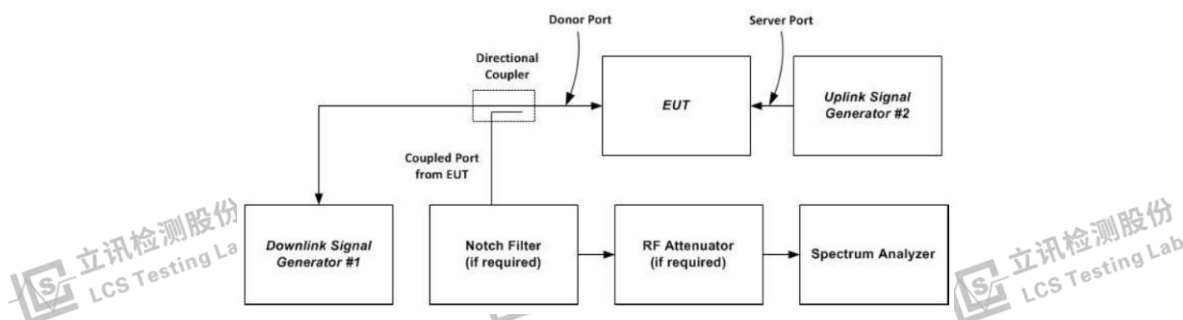
Figure 5 – Variable gain instrumentation test setup
