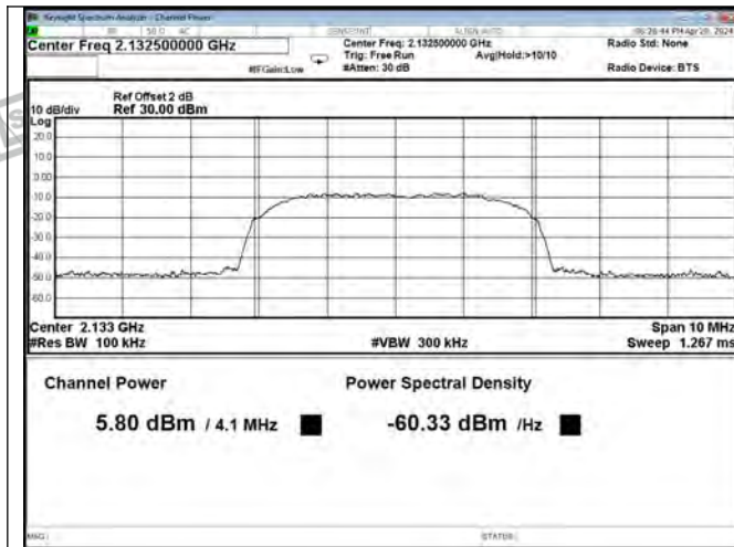
AWS Band AWGN, DL
