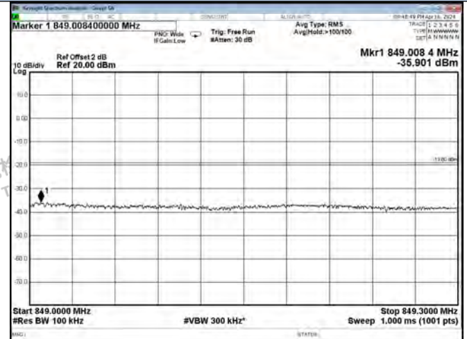
Cellular Band UL-LTE Right Side AGC+10dB
