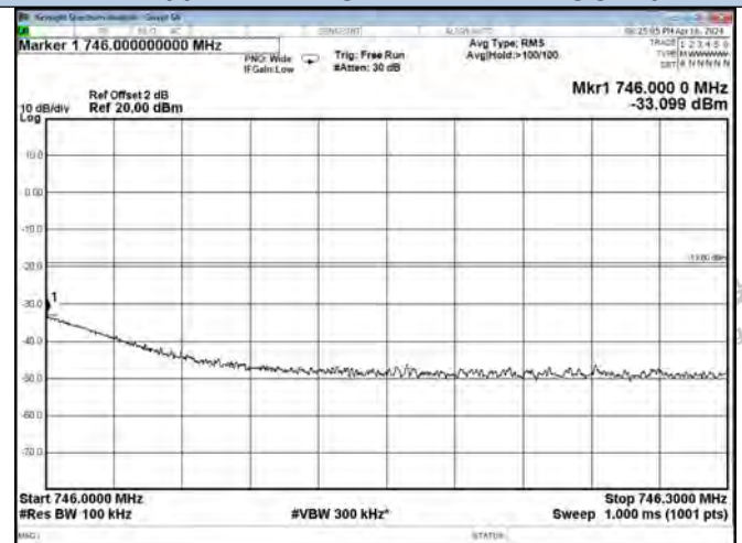
Lower 700 Band DL-GSM Right Side AGC+10dB
