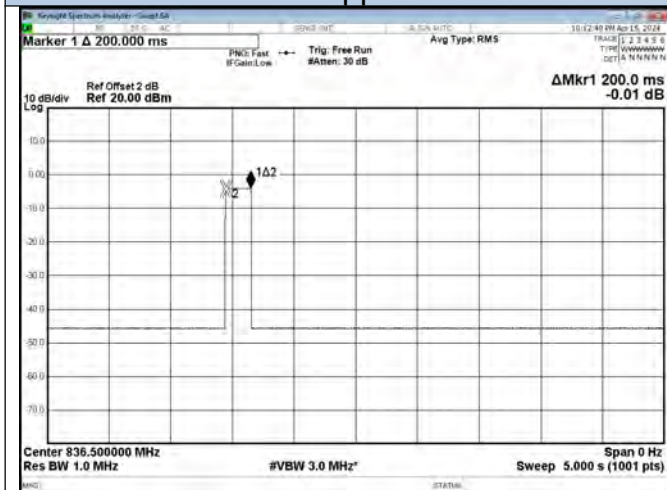
Detection Time-Cellular Band UL
