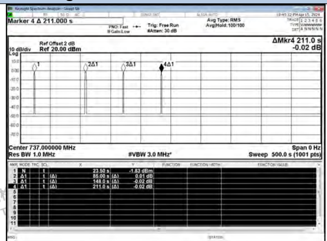
Restarting Time-Lower 700 Band DL
