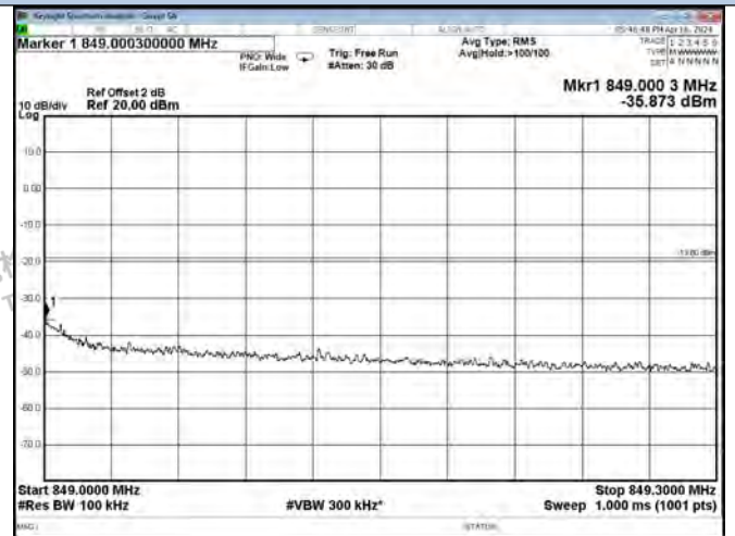
Cellular Band UL-GSM Right Side AGC+10dB
