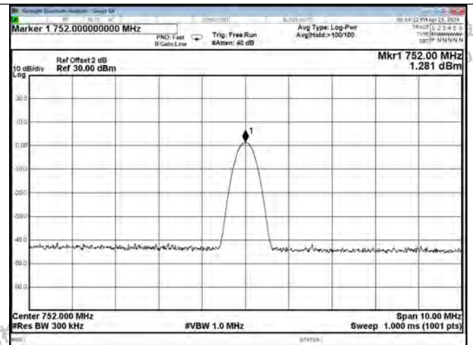
Upper 700 Band CW, DL
