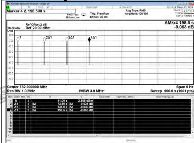
Restarting Time-Upper 700 Band UL
