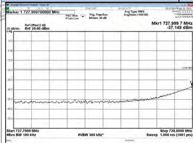
Lower 700 Band DL-GSM Left Side Pre AGC
