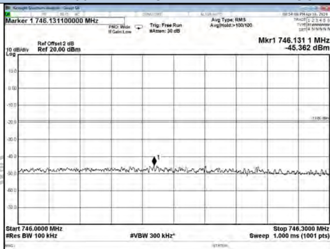
Lower 700 Band DL-CDMA Right Side Pre AGC
