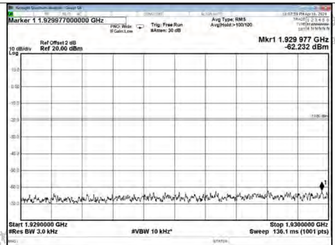
PCS Band DL-LTE Left Side AGC+10dB
