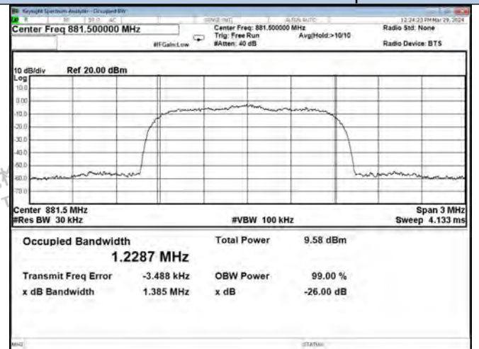
CDMA-Cellular Band DL Output
