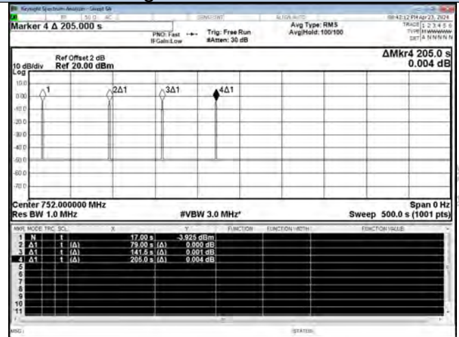
Restarting Time-Upper 700 Band DL
