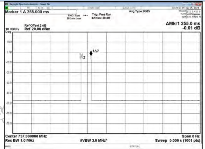
Detection Time-Lower 700 Band DL
