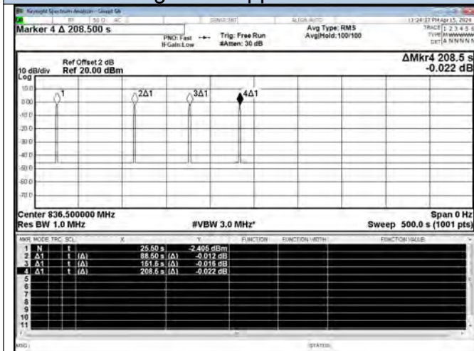
Restarting Time-Cellular Band UL
