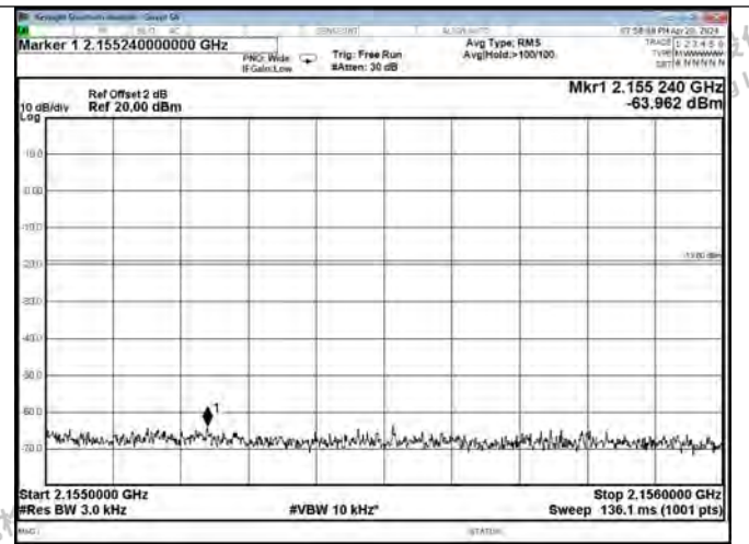
AWS Band DL-LTE Right Side AGC+10dB
