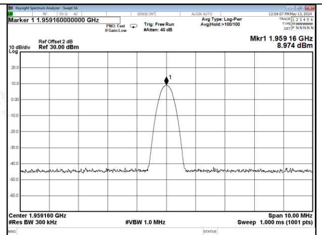
PCS Band CW, DL
