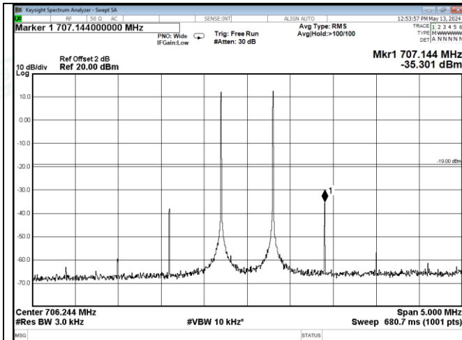
Lower 700MHz band Pre AGC, UL
