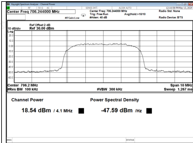
Lower 700MHz Band AWGN, UL
