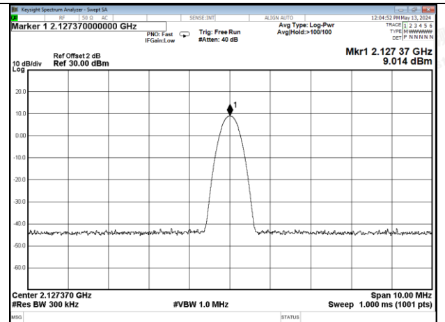
AWS Band CW, DL
