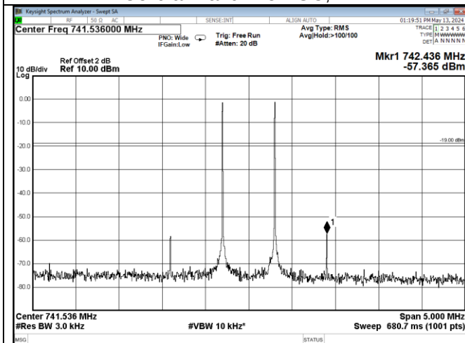
Lower 700MHz band Pre AGC, DL
