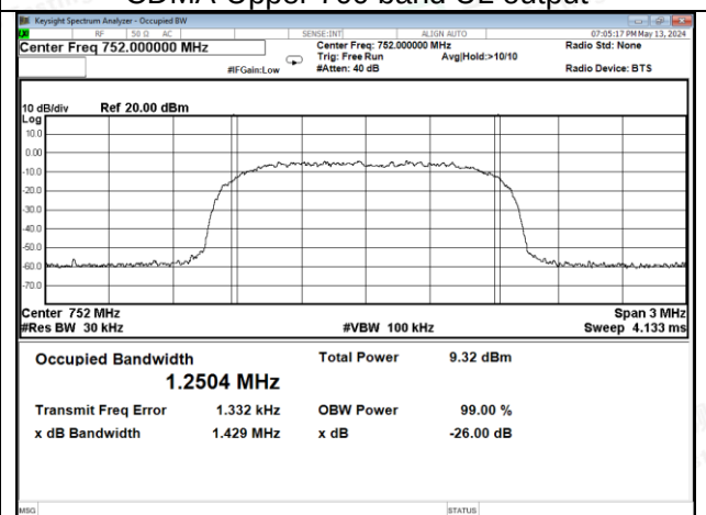
CDMA-Upper 700 band DL output
