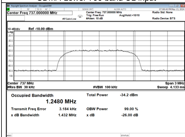
CDMA-Lower 700 band DL input
