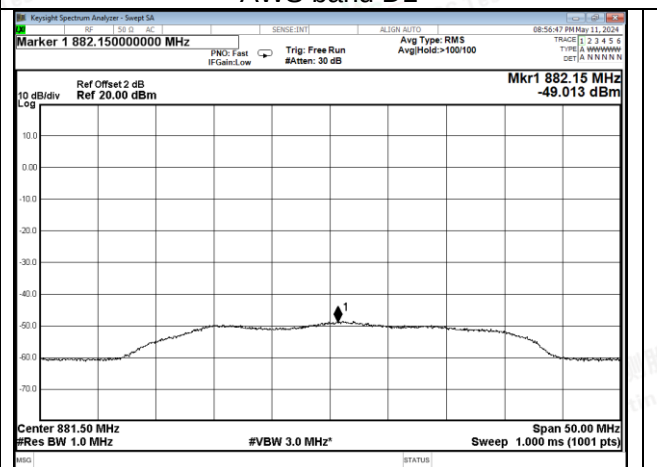
Cellular band DL
