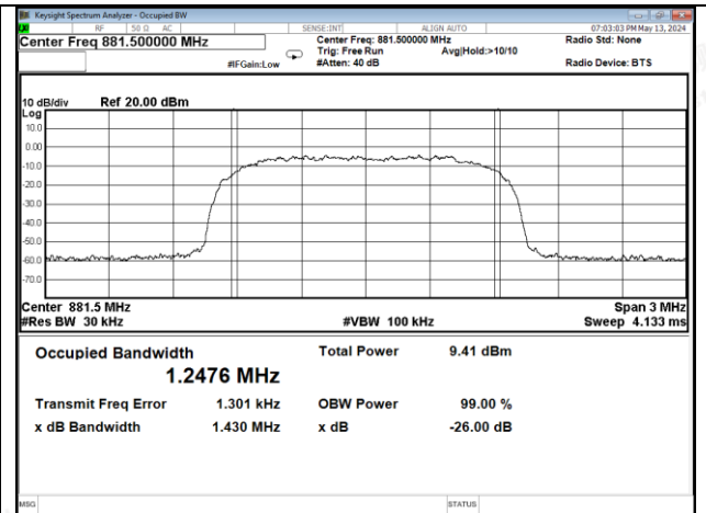
Cellular band DL output
