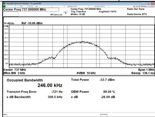
GSM-Lower 700 band DL input
