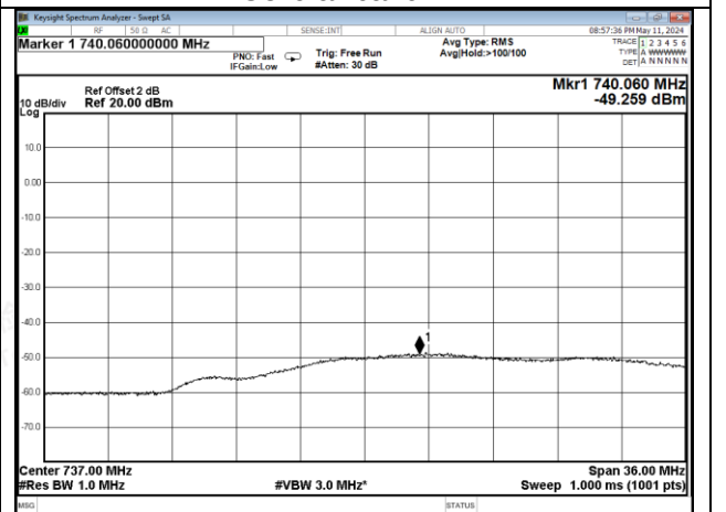
Lower 700MHz band DL
