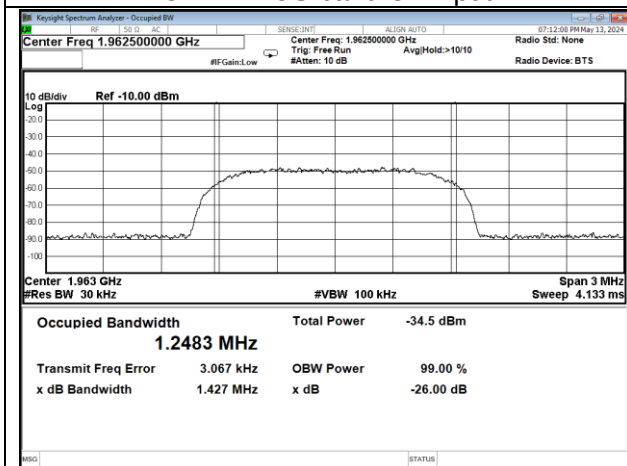
CDMA-PCS band DL input
