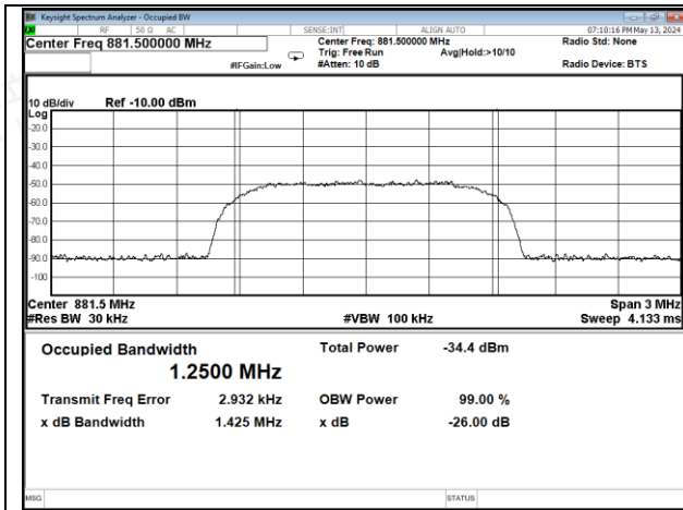
Cellular band DL input
