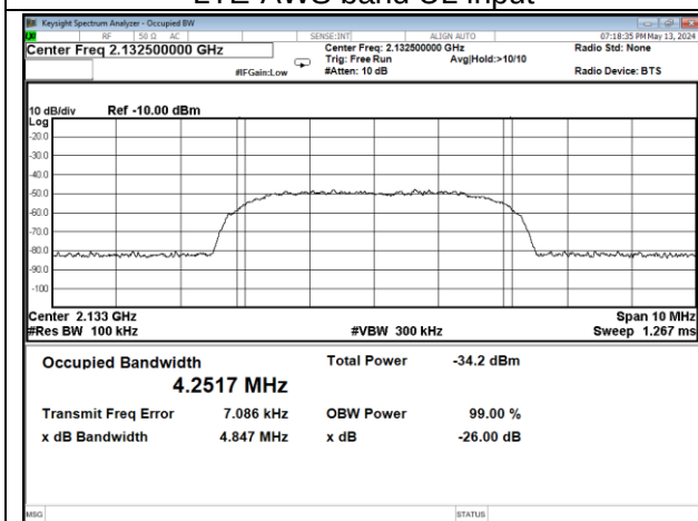
LTE-AWS band DL input
