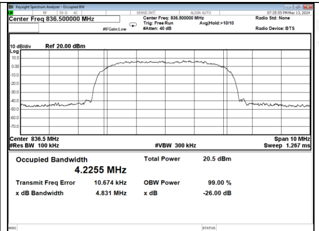
LTE-Cellular band UL output
