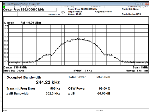
GSM-Cellular band UL input
