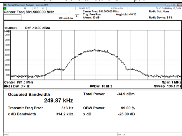
GSM-Cellular band DL input
