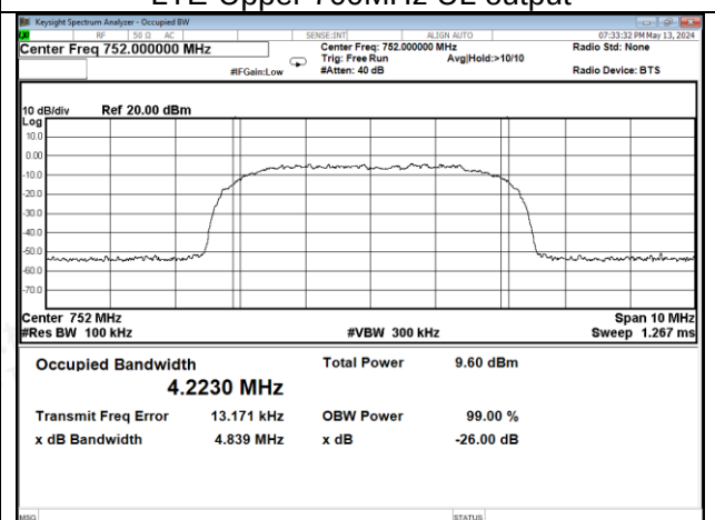
LTE-Upper 700 band DL output
