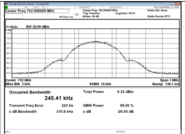
GSM-Upper 700 band DL output
