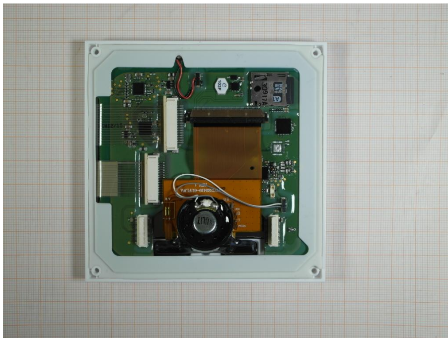
Photo 4 (peripheral board - rear view):
