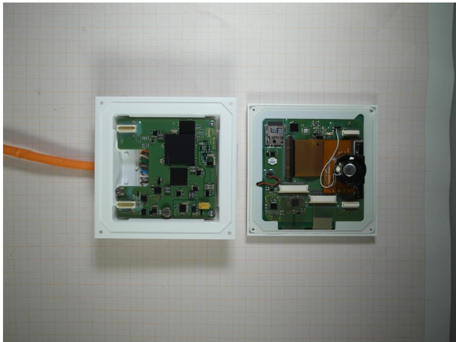
Photo 2 (peripheral board & mainboard):
