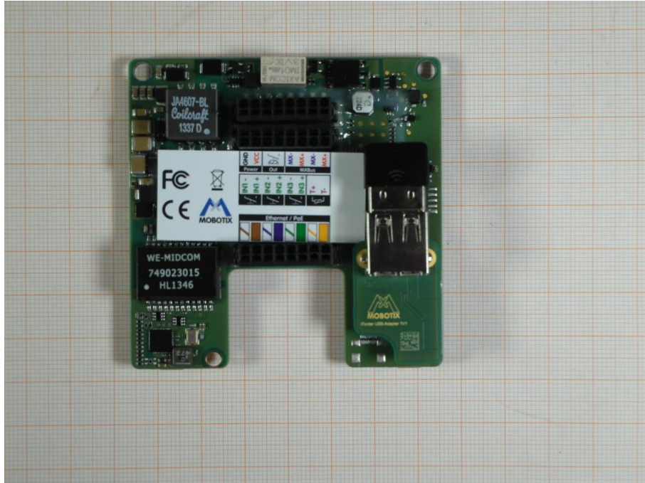
Photo 7 (mainboard - rear view):
