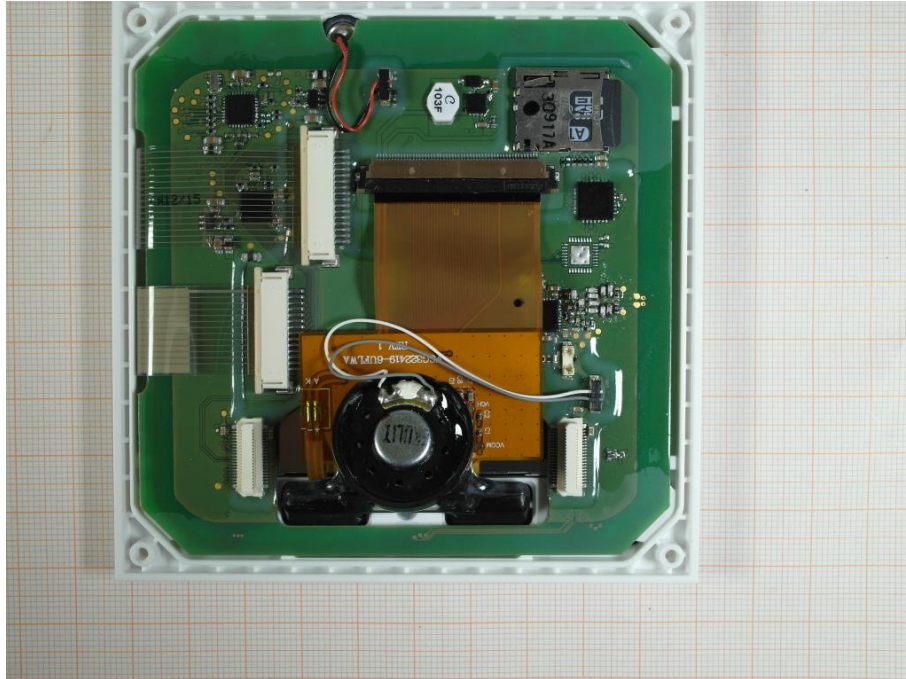
Photo 5 (peripheral board - rear view):
