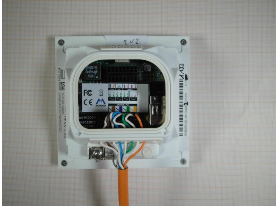
Photo 1 (EUT rear view):
