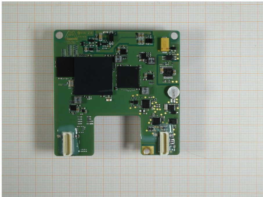
Photo 6 (mainboard - front view):
