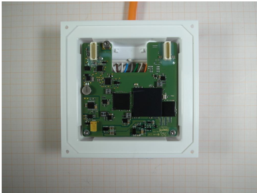
Photo 3 (mainboard front - view):
