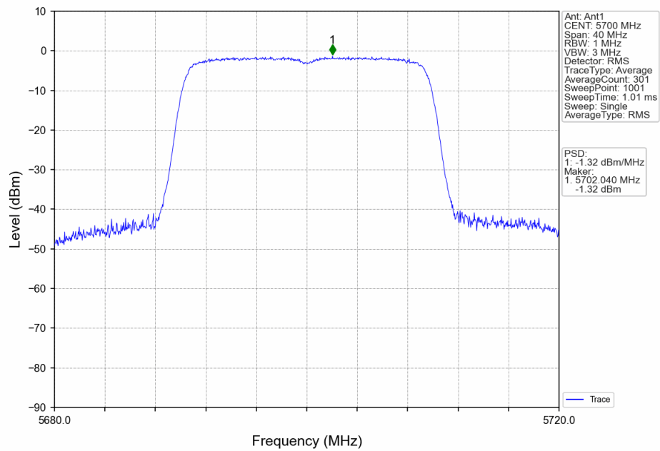
802.11ax(HEW20)_HCH_5700MHz_RU242_Left_Ant1_NTNV
