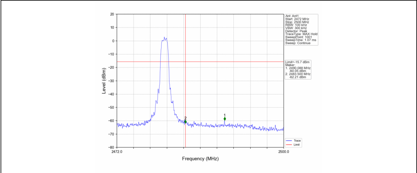
8DPSK_3DH5_HCH_2480MHz_Ant1_NTNV
