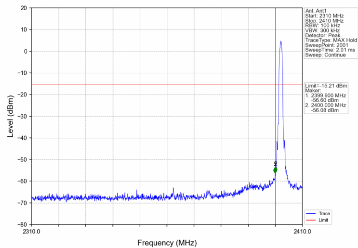
Pi/4DQPSK_2DH5_LCH_2402MHz_Ant1_NTNV
