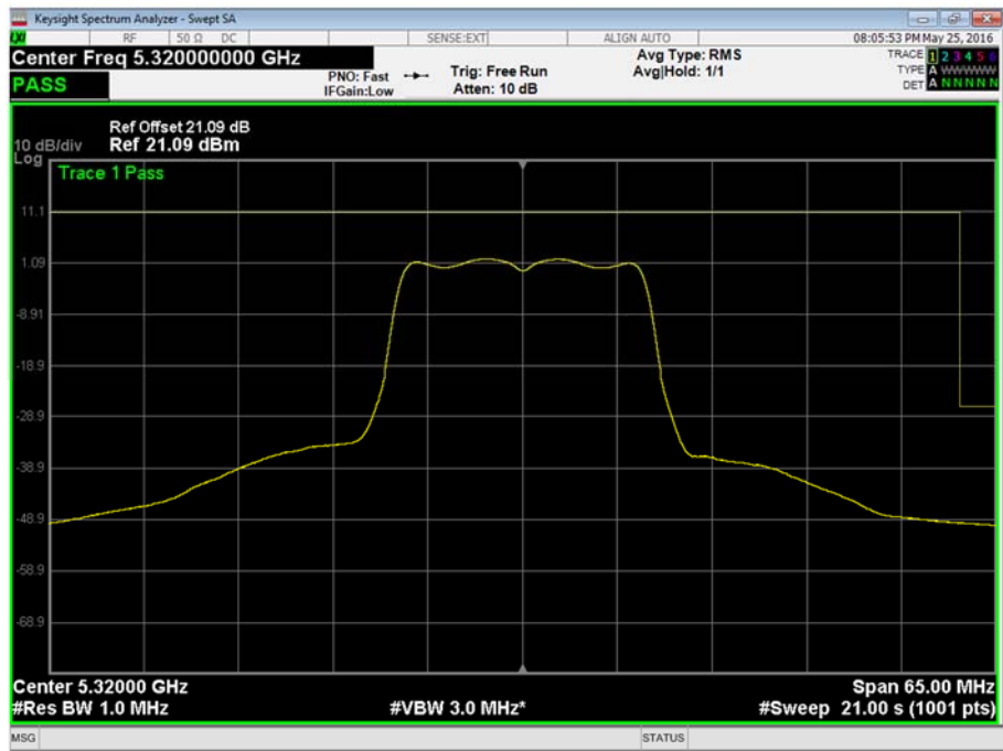
802.11a, 5320 MHz, 0°C, 5.25 V DC, Frequency Band 2, Frequency Stability Plot
