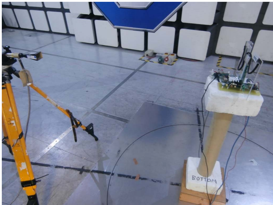
Radiated Emissions 18 GHz to 40 GHz
