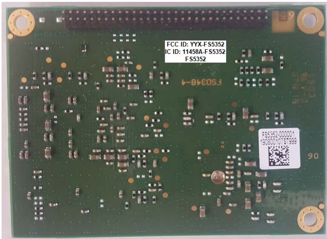
Figure 2: Position of FCC/IC ID label on Minuet 2 module
