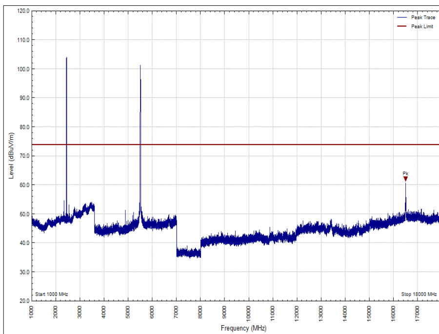
Figure 12 - 1 GHz to 18 GHz - Y Orientation - Peak, Polarisation: Vertical
