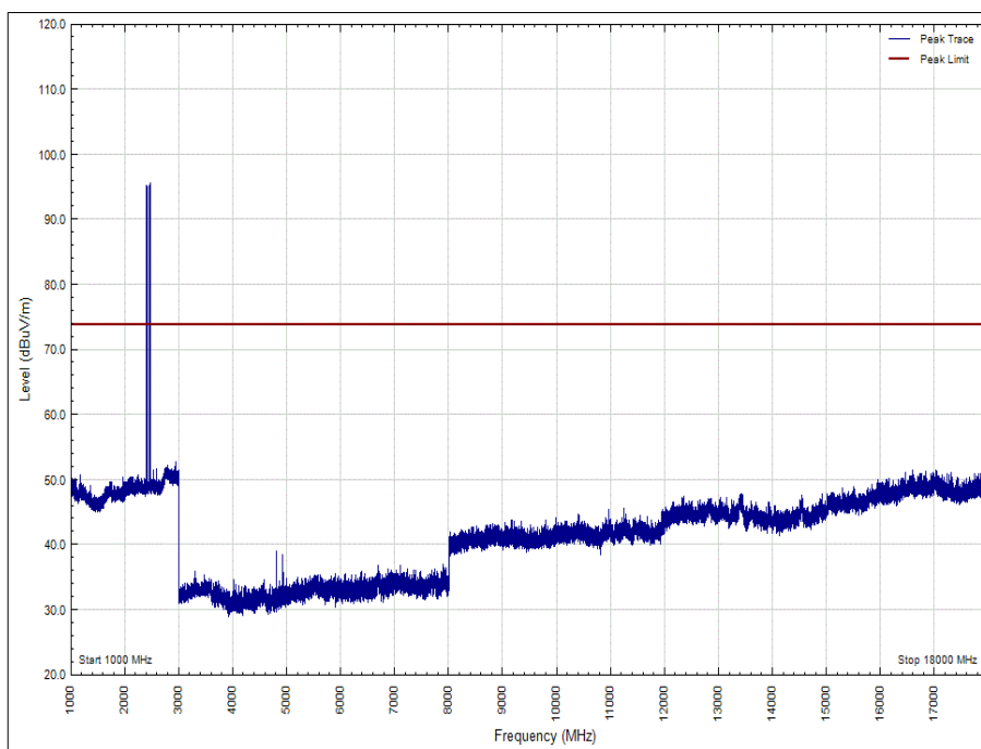
Figure 34 - 1 GHz to 18 GHz - Z Orientation - Peak, Polarisation: Vertical
