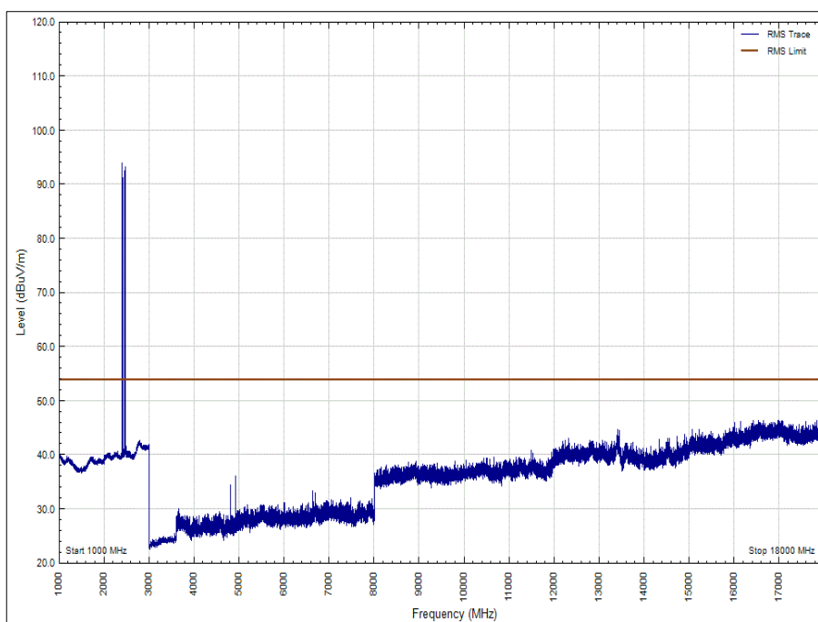
Figure 35 - 1 GHz to 18 GHz - Z Orientation - Average, Polarisation: Vertical
