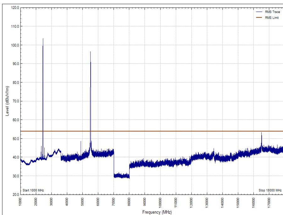
Figure 13 - 1 GHz to 18 GHz - Y Orientation - Average, Polarisation: Vertical
