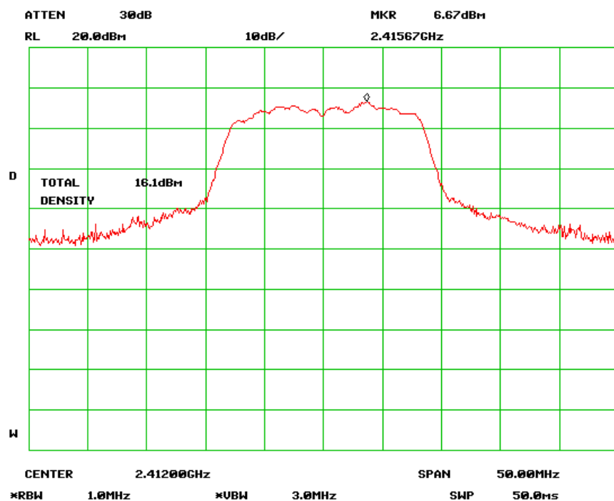
Peak Output Power - Low Channel (802.11g)
