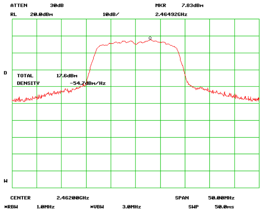
Peak Output Power - High Channel (802.11g)
