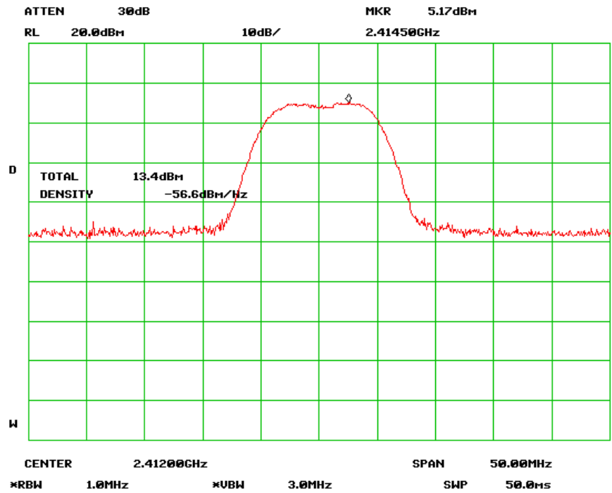
Peak Output Power - Low Channel (802.11b)
