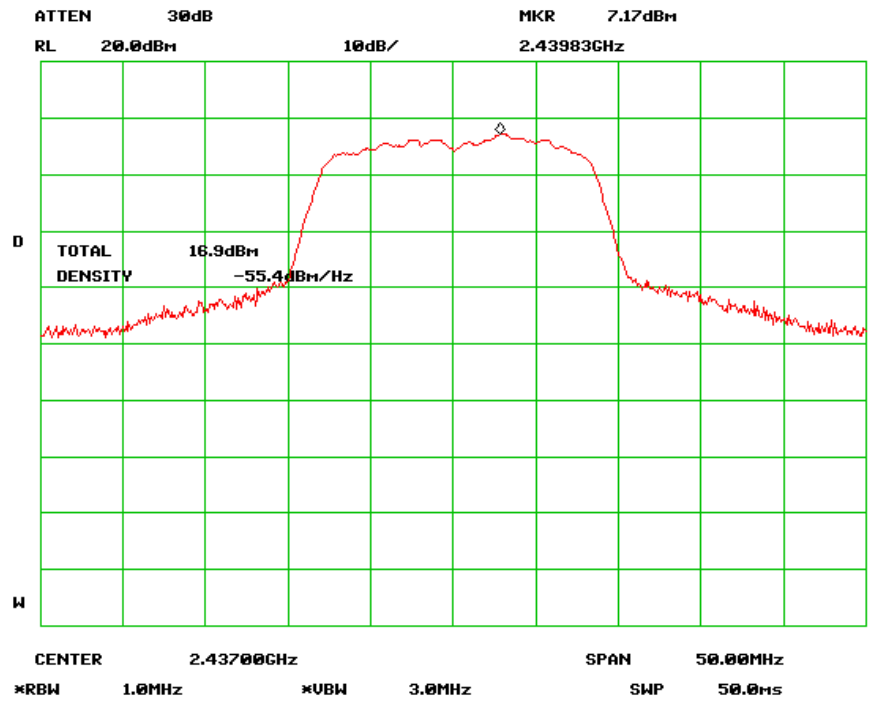
Peak Output Power - Mid Channel (802.11g)
