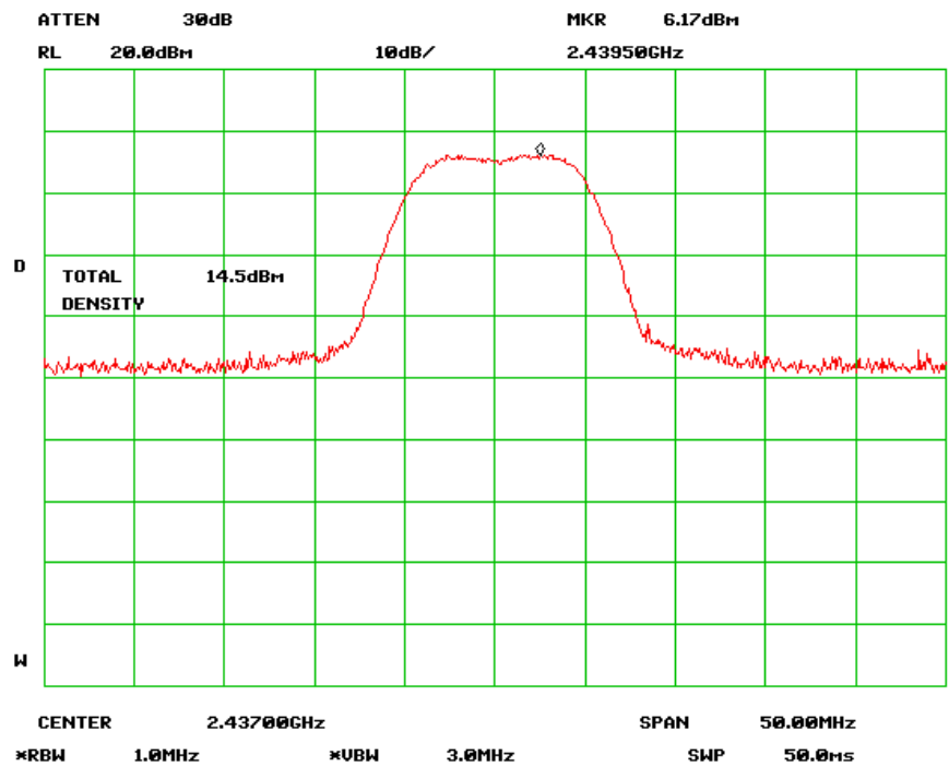
Peak Output Power - Mid Channel (802.11b)
