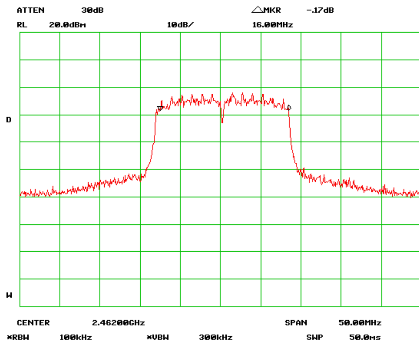
6dB Bandwidth – High Channel (802.11g)
