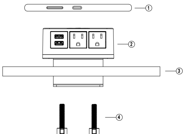
1:MOBILE PHONE; 2. ACQ PS2 QU2 02; 3. BOARD; 4:SCREW NUT
