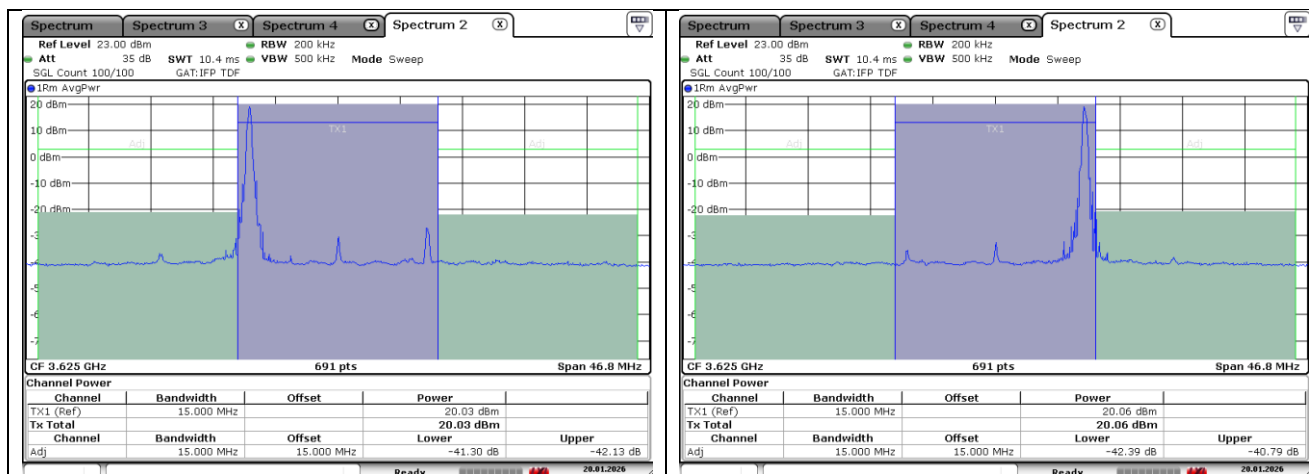
16QAM Middle Channel - 1 RB
