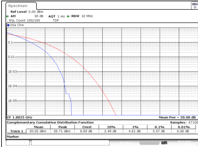
10 MHz Middle Channel - QPSK
