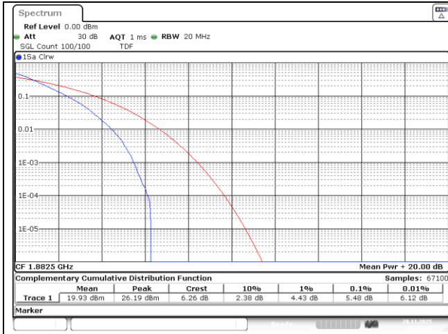
20 MHz Middle Channel - QPSK
