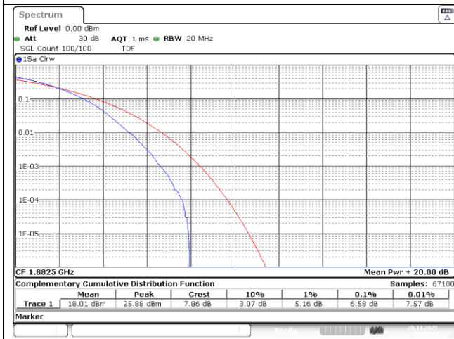
20 MHz Middle Channel - 64QAM
