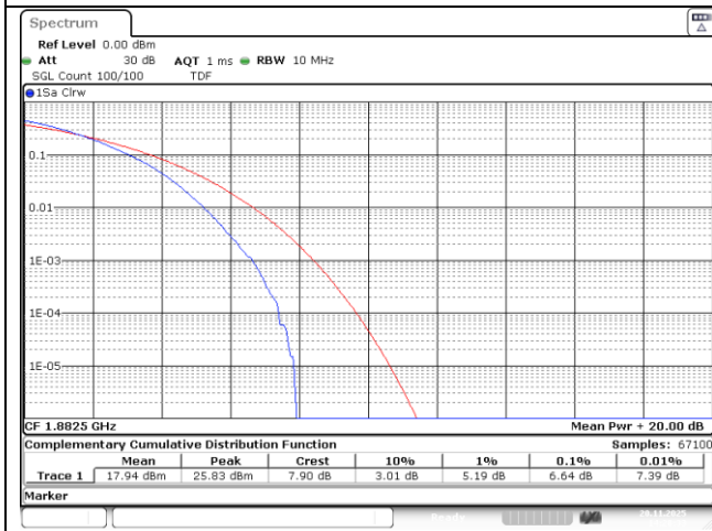
10 MHz Middle Channel - 64QAM
