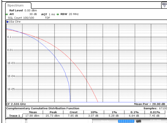
20 MHz Middle Channel - 64QAM
