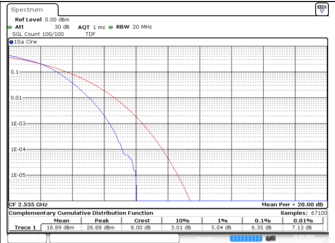
20 MHz Middle Channel - 16QAM
