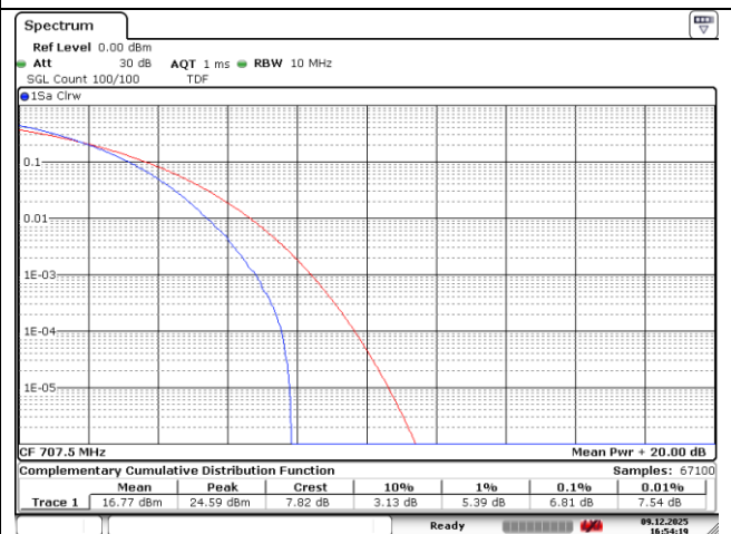
10 MHz Middle Channel - 256QAM
