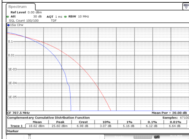
10 MHz Middle Channel - 64QAM
