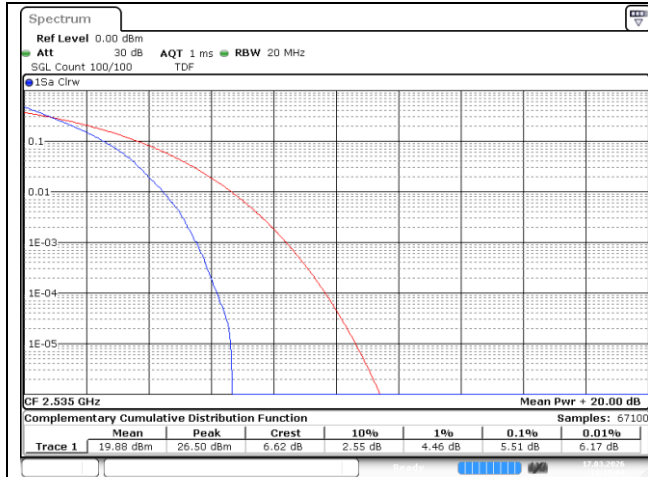
20 MHz Middle Channel - QPSK
