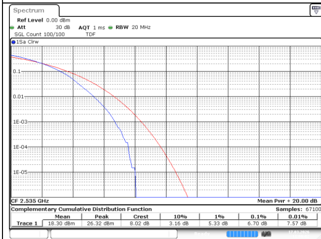
15 MHz Middle Channel - 64QAM
