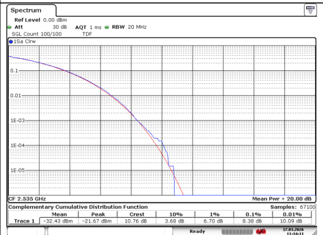
20 MHz Middle Channel - 256QAM
