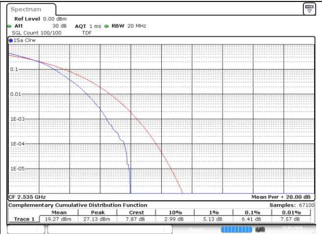
15 MHz Middle Channel - 16QAM
