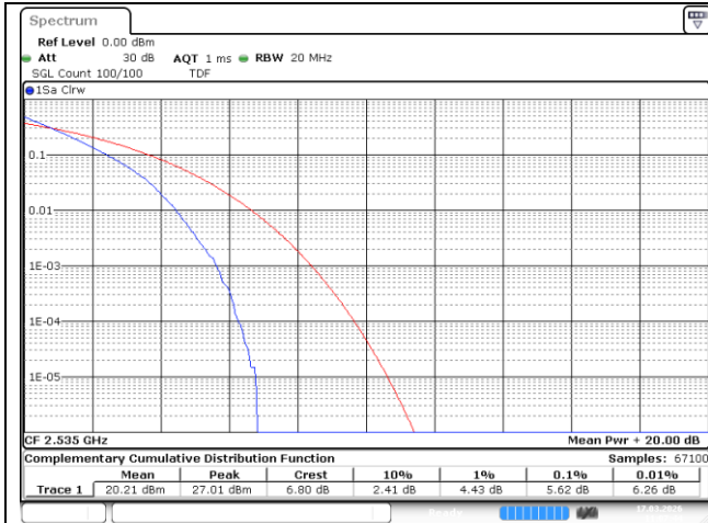
15 MHz Middle Channel - QPSK
