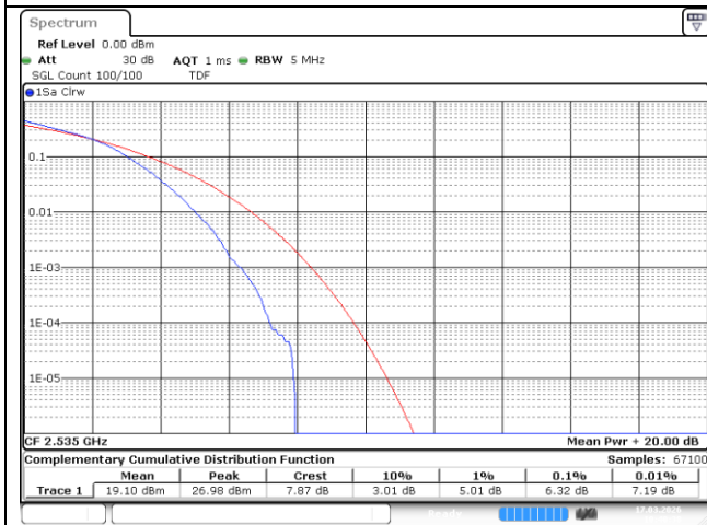
5 MHz Middle Channel - 64QAM
