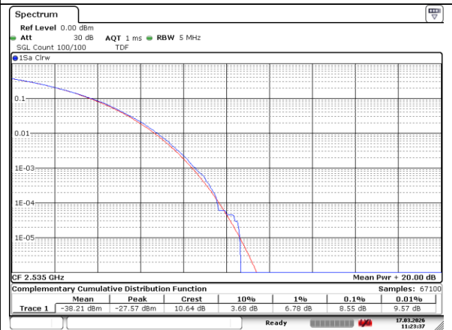
5 MHz Middle Channel - 256QAM
