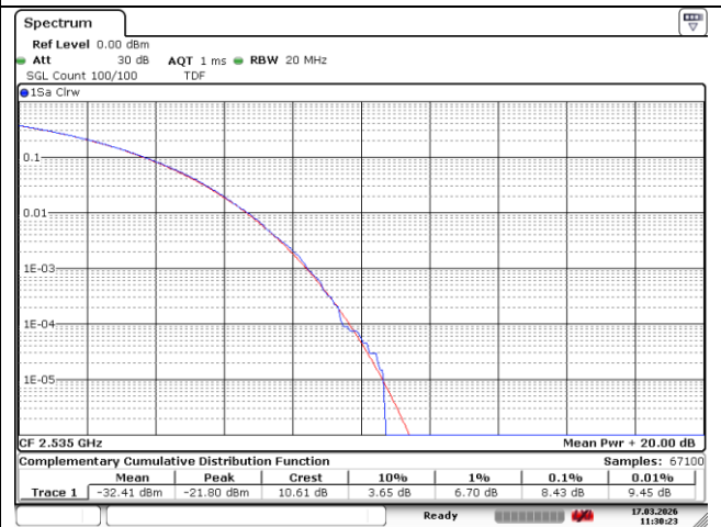
15 MHz Middle Channel - 256QAM
