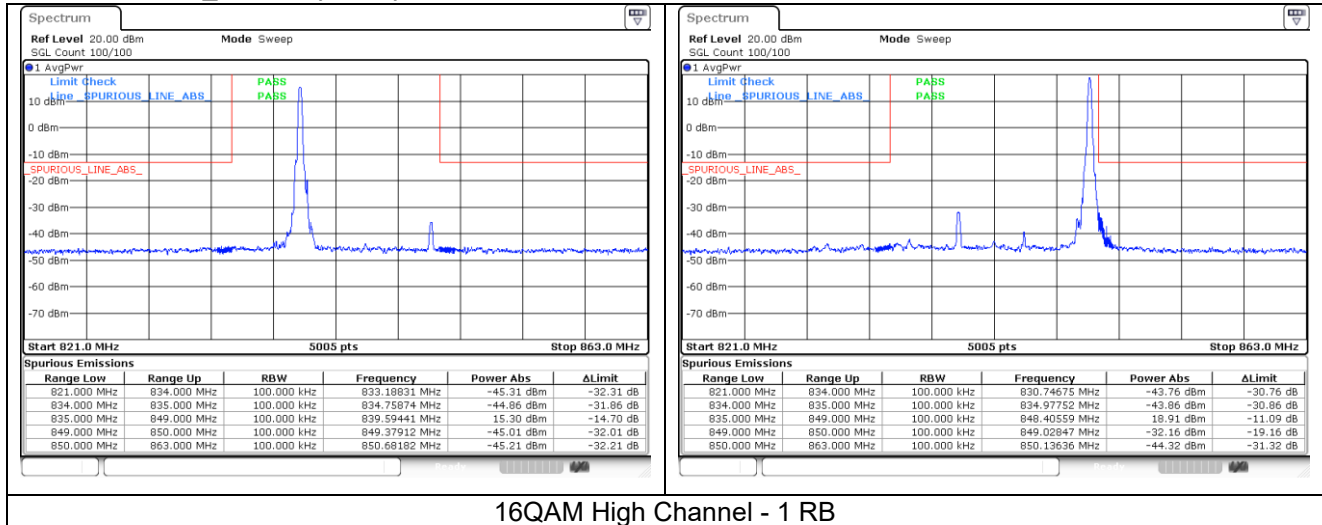
16QAM High Channel - 1 RB
