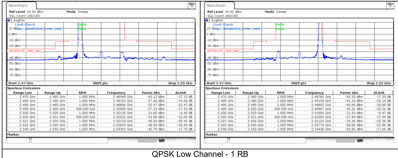
QPSK Low Channel - 1 RB
