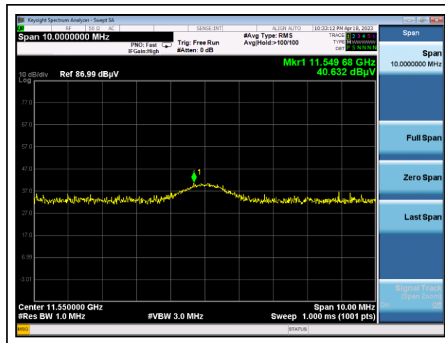
Middle channel 2 nd Spurious (Peak) - Band 3
