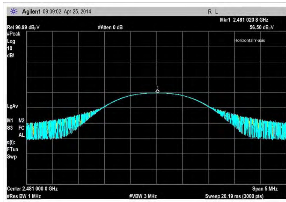
Y-Axis, Horizontal
