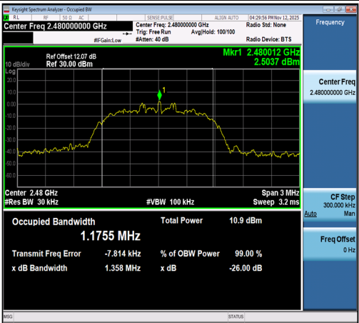
3DH5-Ant1-2480
