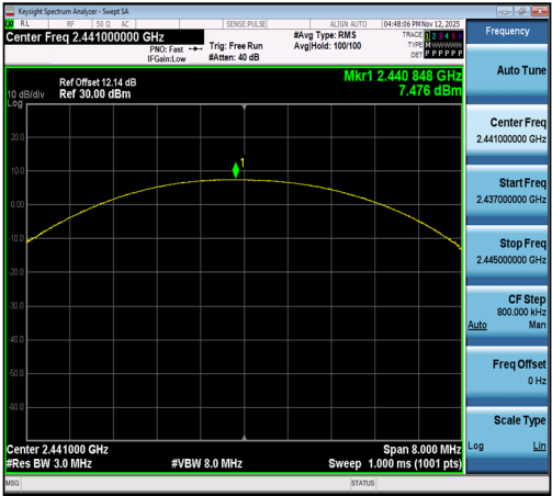
DH5-Ant1-2441-PASS
