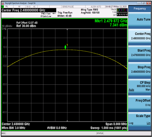
DH5-Ant1-2480-PASS
