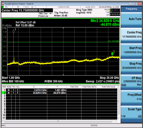
3DH5-Ant1-2480-1000~26500-PASS
