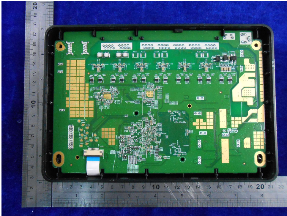
EUT-Uncovered View
