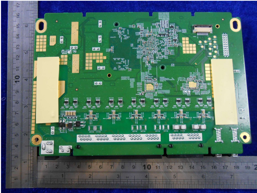
Mainboard-Bottom view
