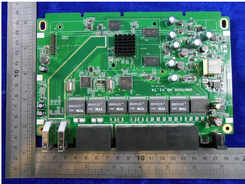
Mainboard-Top view
