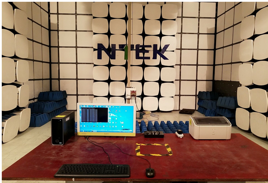
Radiated Emission Test Set-up(Above 1GHz)
