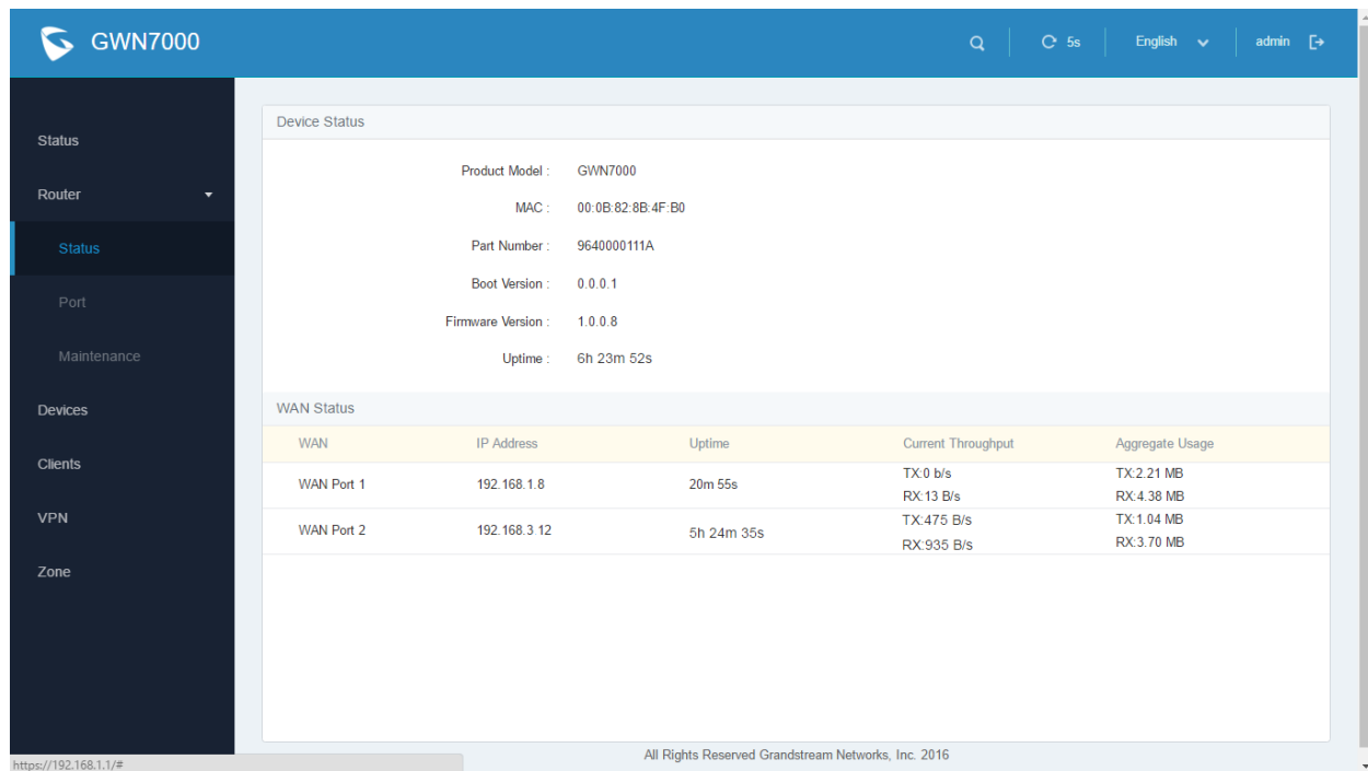
Figure 10: Router's Status
