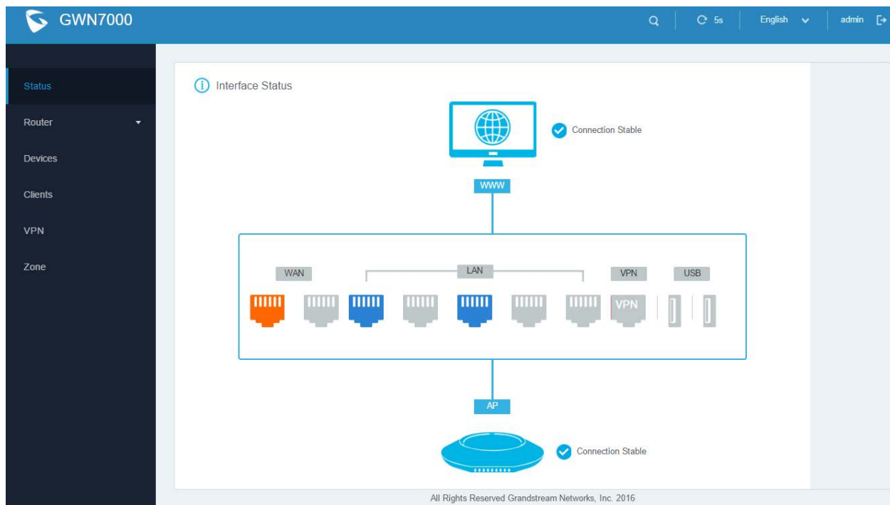
Figure 9: Status Page
