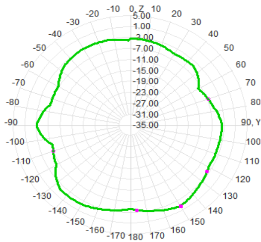
2.4G phi=90deg
