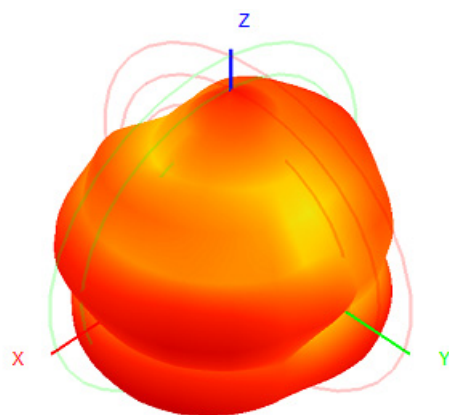
5G 3D
