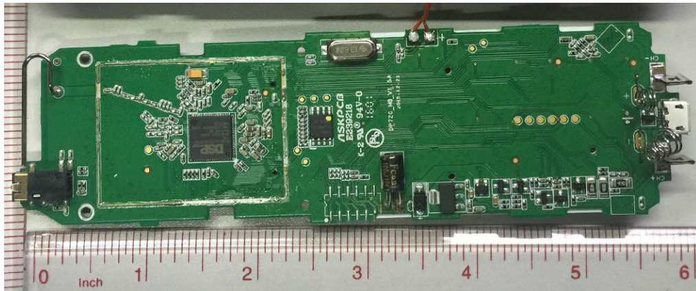
Main board solder side
